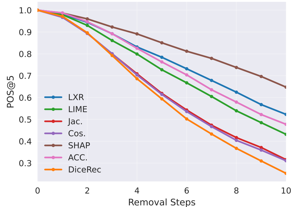
POS@5 vs Removal Steps (0-10)
