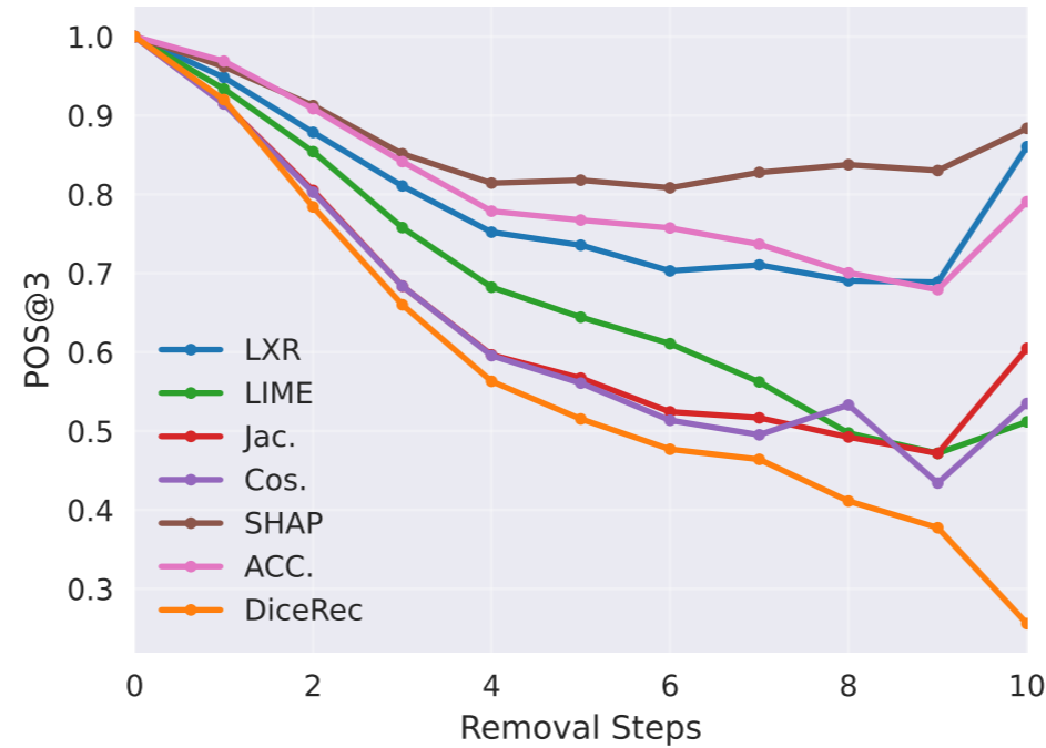
POS@3 vs Removal Steps (0-10)
