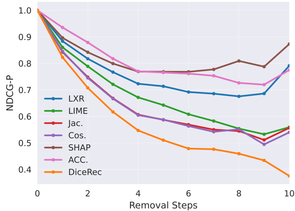
NDCG-P vs Removal Steps (0-10)
