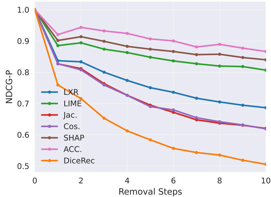
NDCG-P vs Removal Steps (0-10)
