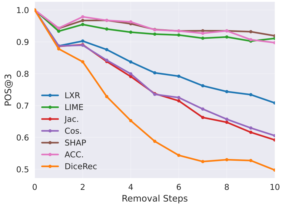
POS@3 vs Removal Steps (0-10)
