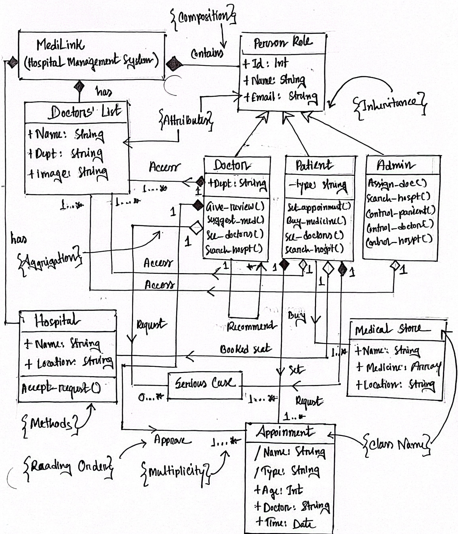
1.1 Figure: Class Diagram of a Hospital Management System
