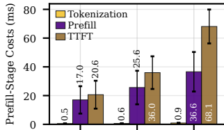
HuggingFace (bf16)
