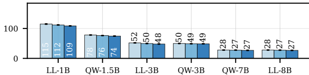
Decode tok/s
