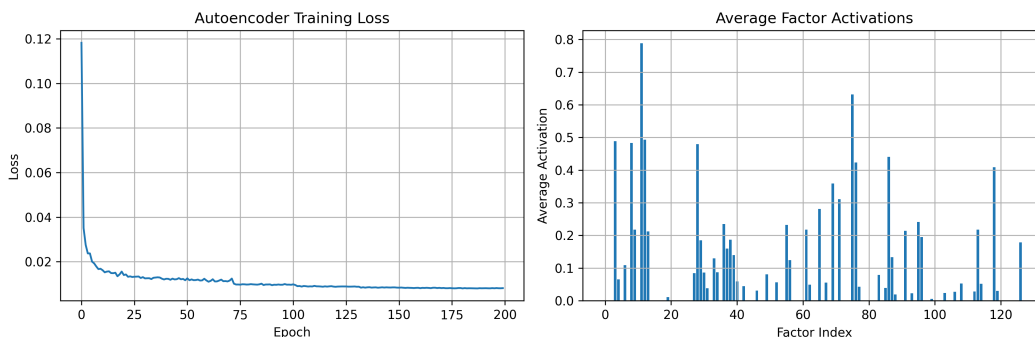
Figure 3: Left: Autoencoder training loss rapidly decreases and plateaus after 50 epochs, indicating stable convergence of the reconstruction and sparsity objectives. Right: Average latent factor activations across 128 neurons show sparse, selective patterns—most factors remain near-zero while a subset exhibits strong activation, consistent with disentanglement and interpretability goals.
