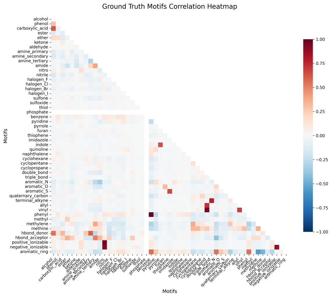
Figure 7: Ground Truth Motif correlations
