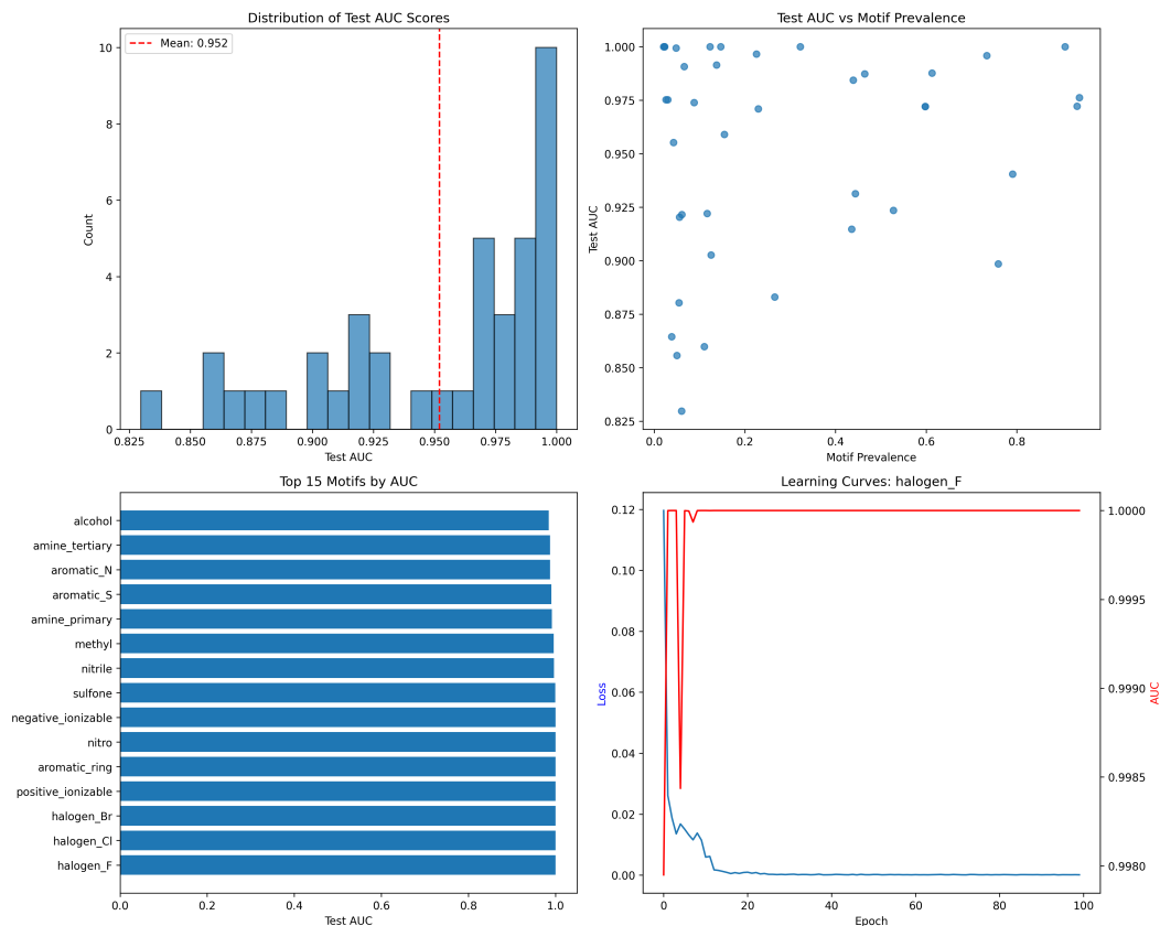
Figure 6: Motif Probe Results
