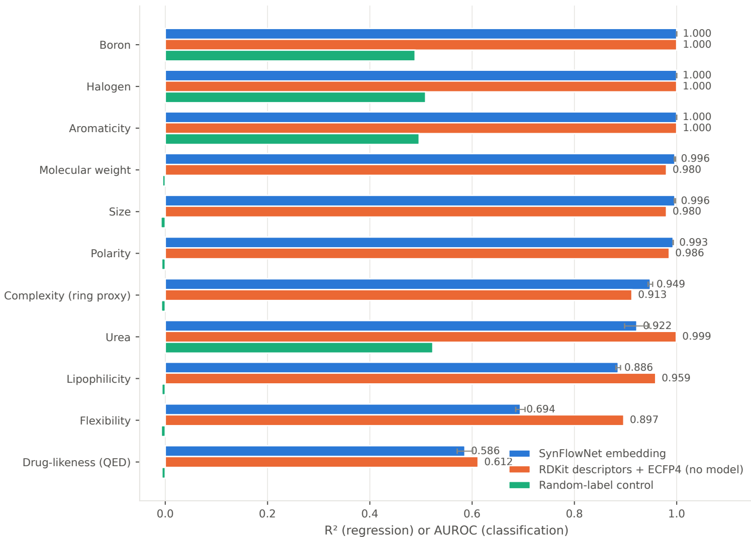
Linear decodability against trivial baselines
