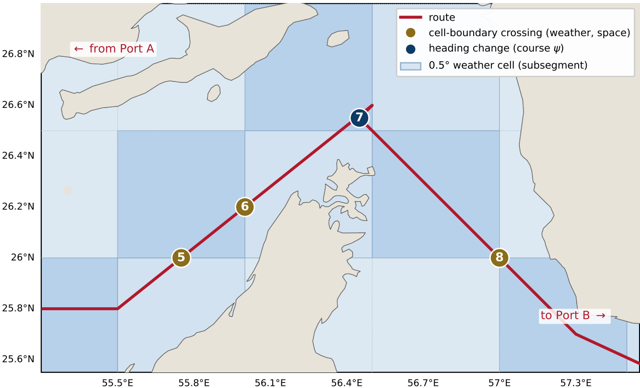
Strait of Hormuz (points 5--8): each cell crossing and the heading change is a speed-change point
