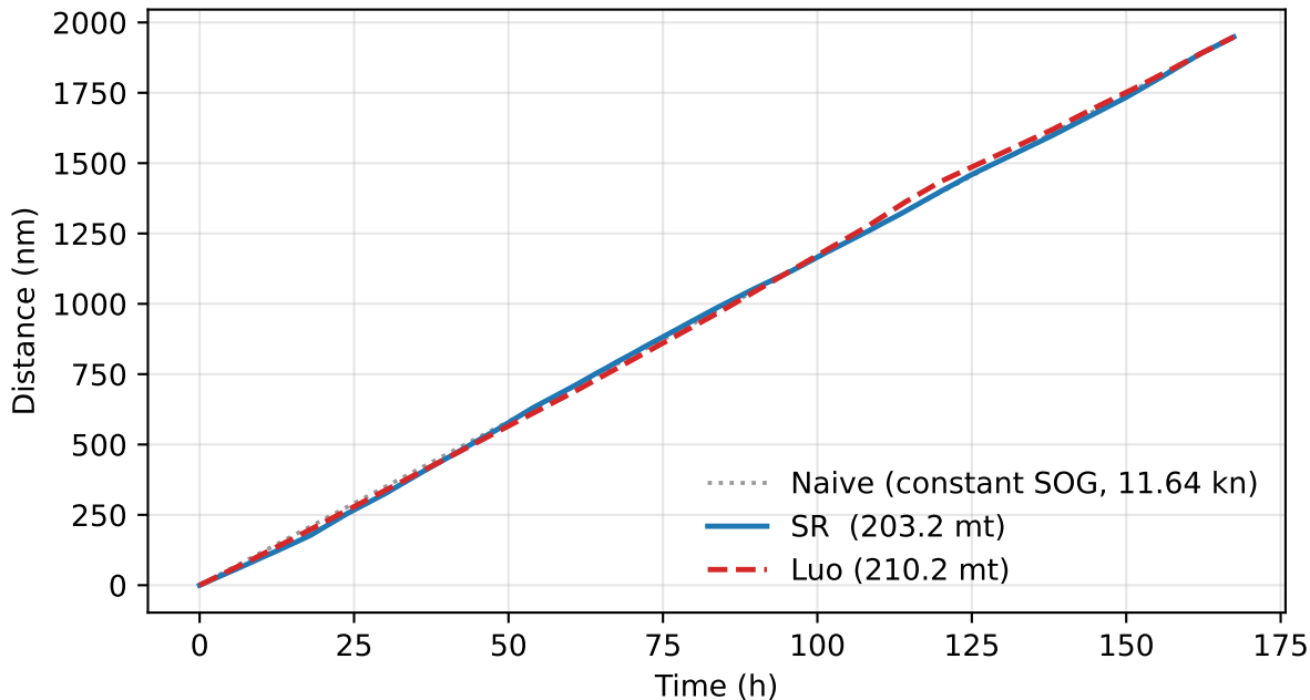
Voyage trajectory — Route 2, voyage 00 (perfect foresight) (slope = SOG)
