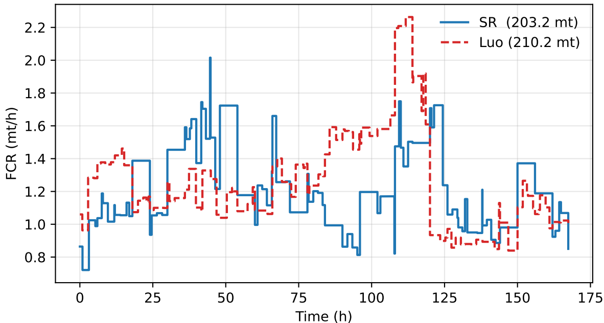
Fuel consumption rate over the voyage Route 2, voyage 00 (perfect foresight)
