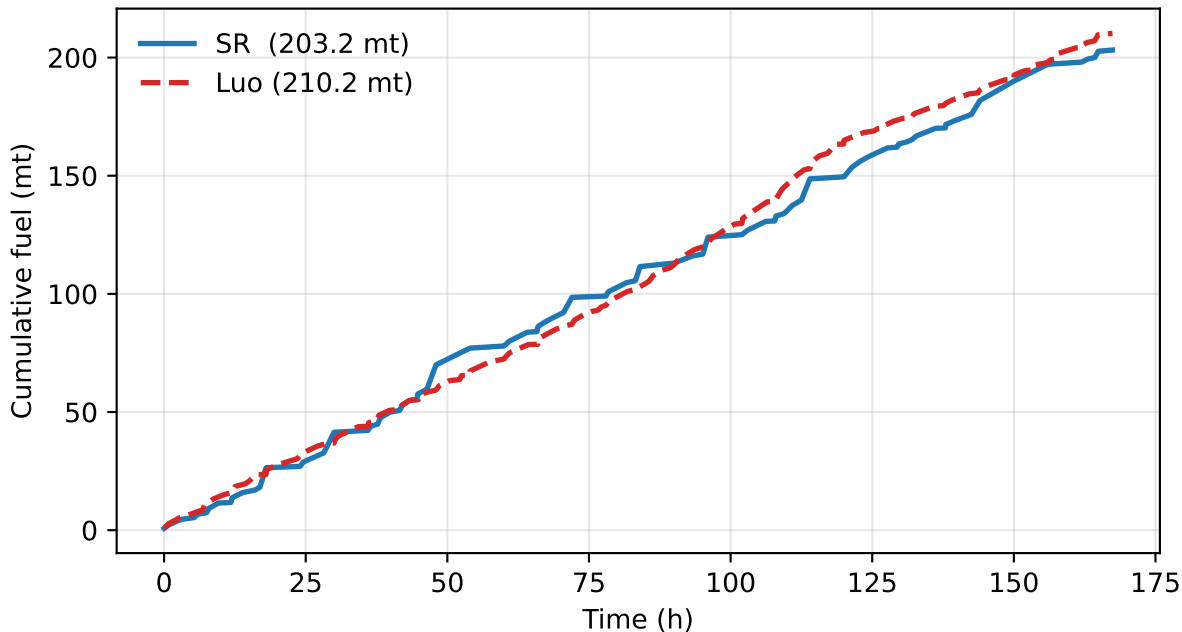
Cumulative fuel over the voyage Route 2, voyage 00 (perfect foresight) — final gap 7.1 mt (3.4 %)
