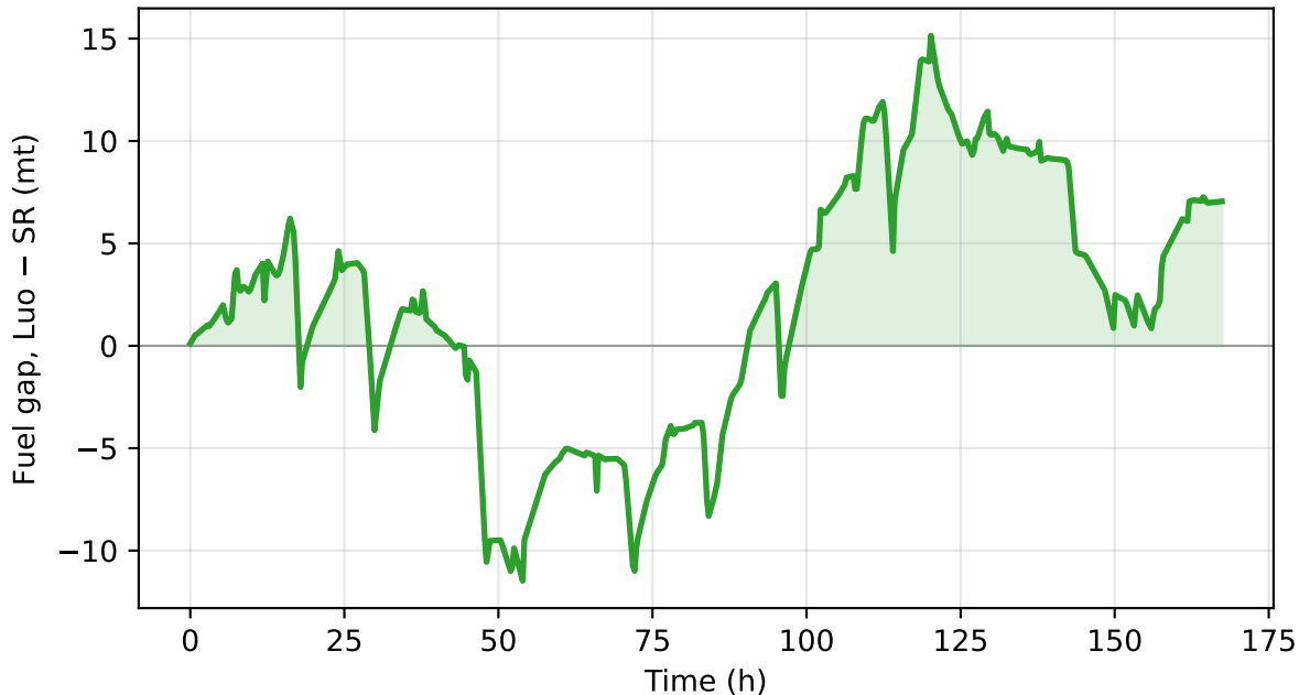
Fuel saved by SR over the voyage Route 2, voyage 00 (perfect foresight) — ends at 7.1 mt (3.4 %)
