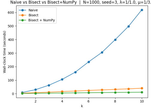
Figure 4.4. Runtime comparison of Naive, Bisect, and Bisect+NumPy simulators for varying rank resolution with N = 1000 jobs
