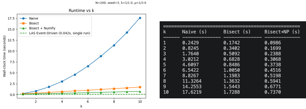
Figure 4.2. Naive vs Bisect vs Bisect + NumPy Runtime on LAS rank data for k=1 to k=10
