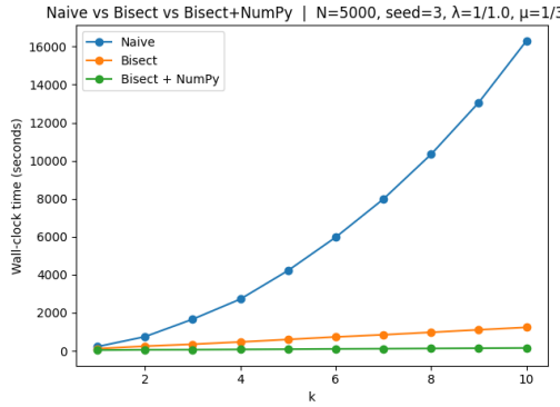
Figure 4.5. Runtime comparison of Naive, Bisect, and Bisect+NumPy simulators for varying rank resolution with N = 5000 jobs
