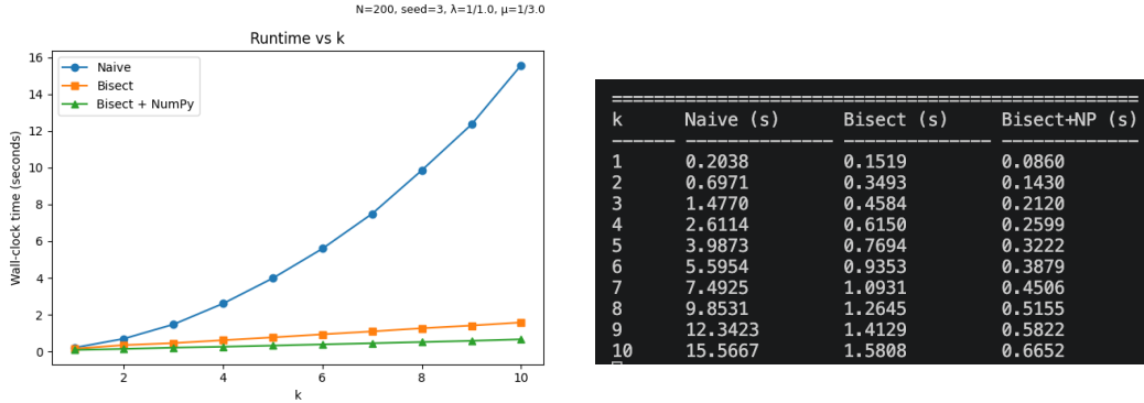
Figure 4.1. Naive vs Bisect vs NumPy+Bisect Runtime on pre-provided rank data for k=1 to k=10
