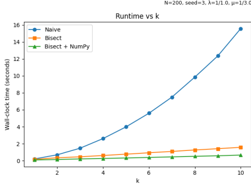
Figure 4.3. Runtime comparison of Naive, Bisect, and Bisect+NumPy simulators for varying rank resolution with N = 200 jobs.
