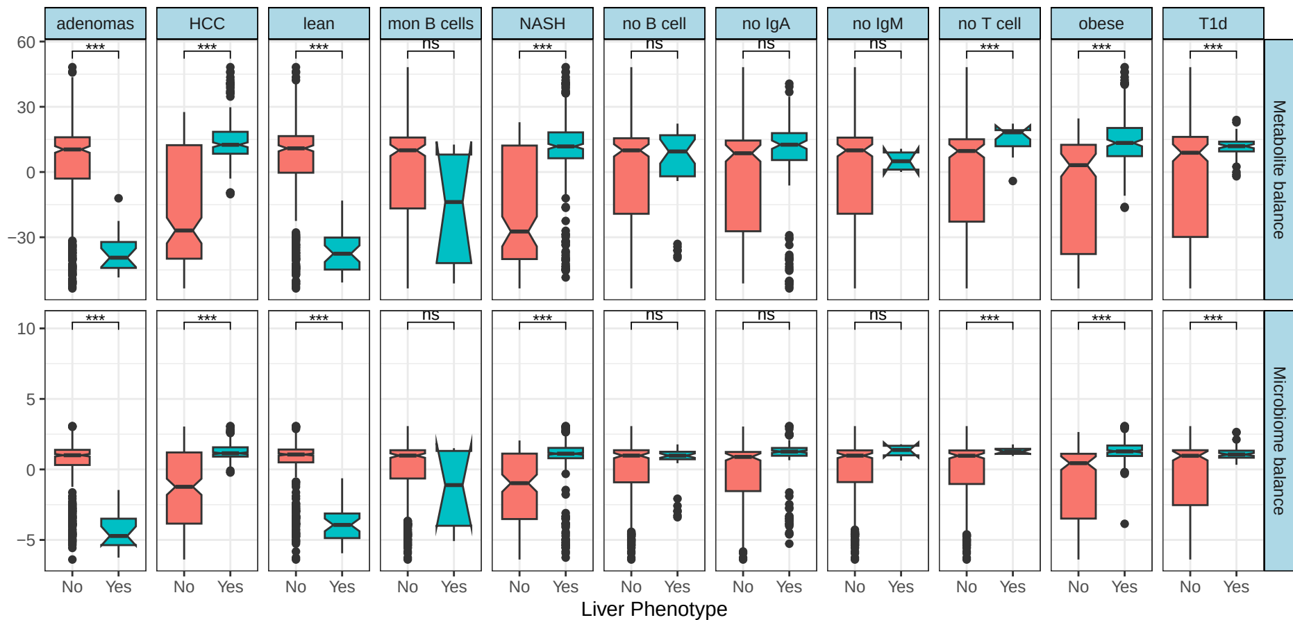
Boxplot with Statistical Significance
