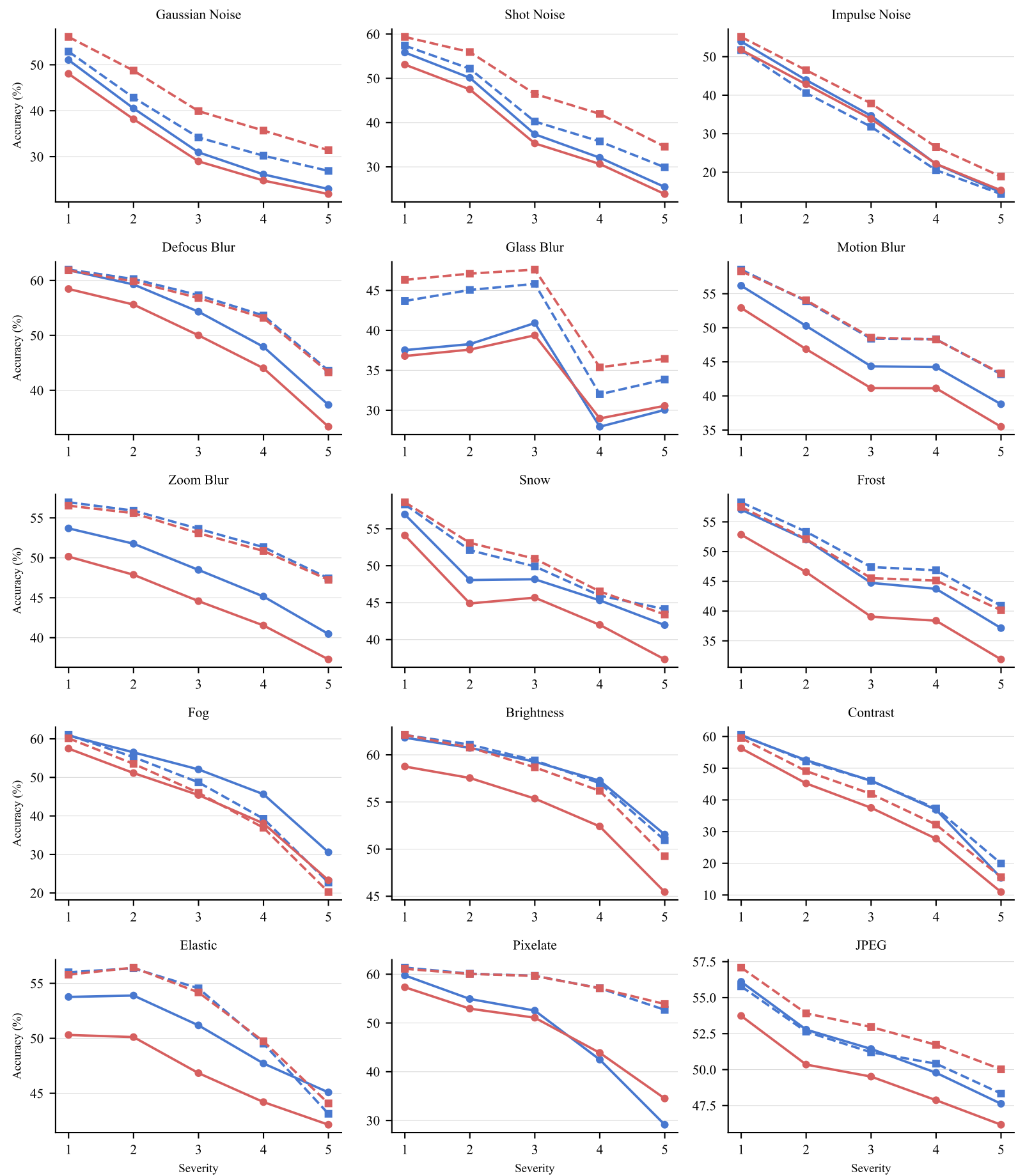
CIFAR-100-C — Per-Corruption Accuracy vs. Severity
