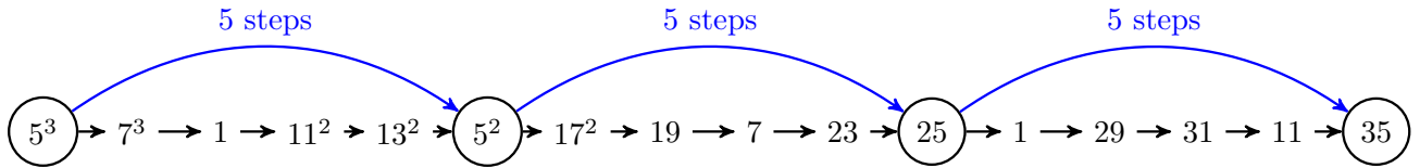
FIGURE 3. Hop-step for prime 5
