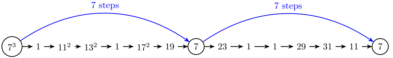
FIGURE 5. Hop-step for prime 7
