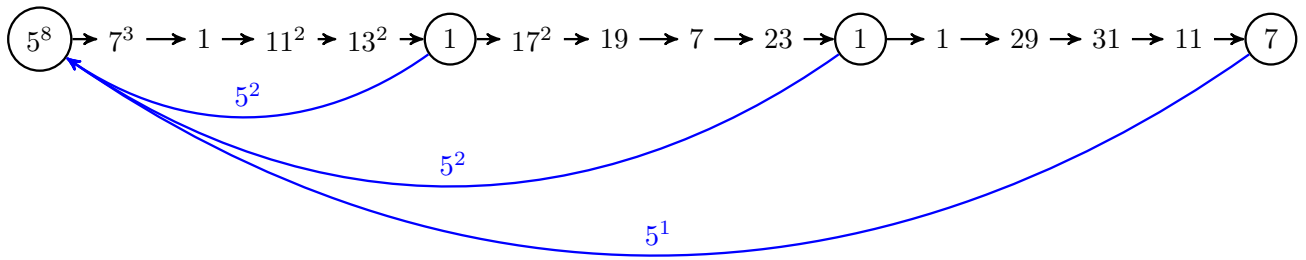
FIGURE 3. Hop-step for prime 5
