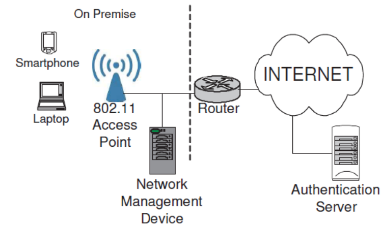
Fig 1. Mobile Internet access using Wi-Fi hotspots
