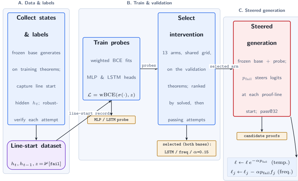
Figure E.1: Probe-guided generation pipeline. Only the probe ( < 3\text{M} parameters) is trained; the prover weights are frozen. Symbols: h_t is the line-start hidden state, z the robust fail label, p_{\text{fail}} the probe’s failure probability, \ell the logits, \alpha the steering strength, f_j the token frequency.
