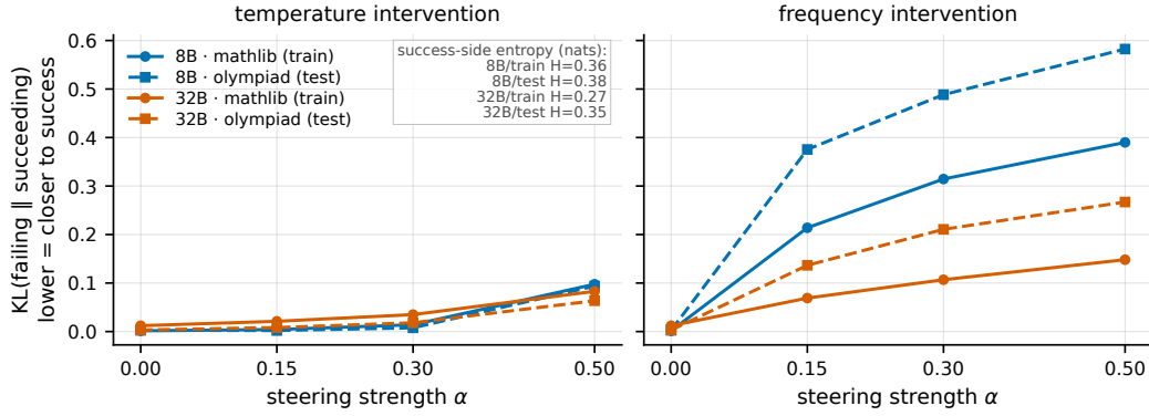
Figure F.4: Steering moves failing generations away from success, not toward it. Kullback–Leibler divergence between the failing attempts’ next-token distribution after steering and the succeeding attempts’ distribution, against steering strength \alpha , over exactly the grid the validation contest searched. Lower would mean steering makes failing generations look more like succeeding ones; seven of the eight curves rise from \alpha=0 , and the eighth dips negligibly at \alpha=0.15 before rising. Curves use an oracle probe ( p_{\text{fail}}=1 on failed attempts); the trained MLP and LSTM curves lie essentially on top of them. Both sides are mean rank profiles : each next-token distribution is sorted into decreasing probability order before averaging, so the curves compare distribution shape at matched ranks rather than matched tokens.
