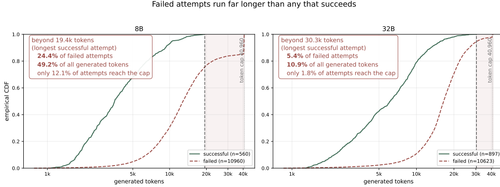
Figure F.2: Failed attempts run far longer than any that succeeds. Empirical CDF of generated tokens per attempt, MathOlympiad-Bench pass@32, base models, split by the robust verdict. The dashed line is the longest attempt that ever verified, 19.4k tokens on 8B and 30.3k on 32B; the shaded region is everything beyond it. Only 12.1% of 8B attempts and 1.8% of 32B attempts reach the 40,960-token cap, but 24.4% and 5.4% of failures run past anything that has ever succeeded, and those attempts consume 49.2% and 10.9% of all generated tokens. Compressibility is not plotted because it is largely a second view of the same length signal (§6.4).
