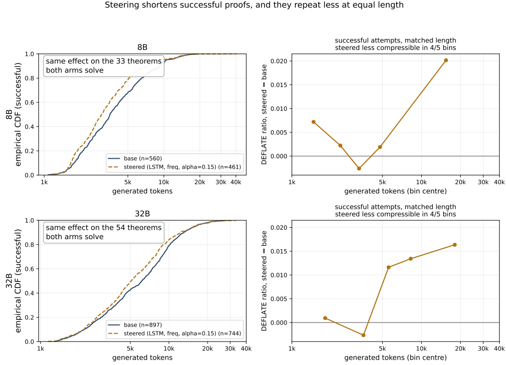
Figure F.3: Steering shortens successful proofs, and they repeat less at equal length. Successful attempts only. Left: the steered arm’s median successful proof is 15–18% shorter (3,550 → 3,032 tokens on 8B, 6,159 → 5,080 on 32B); restricted to the 33 and 54 theorems both arms solve the effect is the same, so it is not an artifact of which theorems survived. Right: because shorter text is mechanically less compressible, the claim needs a control, so the DEFLATE ratio is compared inside matched length bins; steered output is less compressible in 4 of 5 bins on both bases, and the gap grows with length, which is what a frequency penalty should do. This is evidence that the intervention acts, not that it helps: the same arm closes fewer goals, 41 → 35 on 8B and 60 → 59 on 32B.
