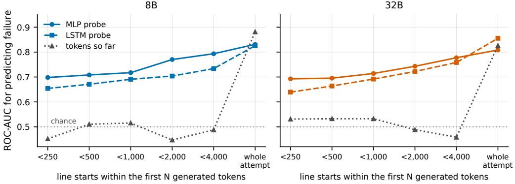
Figure 6.1: The signal is available early; length is not. Per-line ROC-AUC restricted to the line starts falling inside the first N generated tokens. The probes are well above chance from the first 250 tokens, while the online length feature, how many tokens have been generated so far, sits at chance until a runaway has already happened. Inside a truncated window that feature is near-degenerate by construction, so chance is its expected value; the point is that position carries no early information. The rightmost point is not an online comparison: over a whole attempt “tokens so far” becomes the attempt’s total length, knowable only once it has ended, so it is a retrospective ceiling rather than a feature a controller could use.
