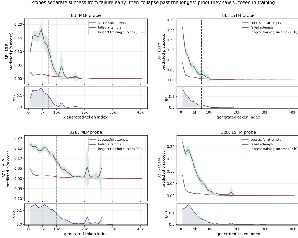
Figure F.1: Probes separate success from failure early, then collapse past the longest proof they saw succeed in training. Mean predicted p(\text{success}) against generated-token index on MathOlympiadBench, with 90% intervals; the strip below each panel is the success-minus-failure gap. Two readings must be kept apart. The curves sit low throughout, peaking at 0.09–0.27: out of domain the probes are badly calibrated , which is expected because the training theorems were easier and succeeded far more often. The gap between the curves is discrimination , and it is large early. The dashed line marks the longest successful training attempt (7,303 generated tokens on 8B, 9,932 on 32B); across it the mean gap falls by between 6\times and 40\times . It does not vanish there: the gap first reaches zero between 10,752 and 28,160 tokens, 1.5 to 2.9 times further out.
