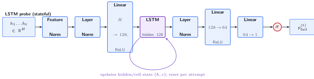
Figure E.3: LSTM probe head (stateful) . Its input is the line-start hidden state h_t alone, \in \mathbb{R}^H , one line start at a time; the LSTM’s own hidden and cell state (h, c) is updated at each line start and reset at the start of each attempt, so the head effectively sees the prefix h_1 \dots h_t . H is the LLM hidden size (4096/5120 for 8B/32B); feature normalization applies the mean and standard deviation stored in the checkpoint, LN is layer normalization, ReLU the rectified-linear activation and \sigma the logistic function. The head has 0.67/0.81M parameters and emits the failure probability p_{\text{fail}}^{(t)} for that line start.
