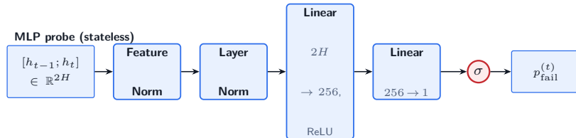
Figure E.2: MLP probe head (stateless). Its input is the previous and current proof-line-start hidden states concatenated, [h_{t-1}; h_t] \in \mathbb{R}^{2H} , with H the LLM hidden size (4096/5120 for 8B/32B). Feature normalization applies the mean and standard deviation stored in the checkpoint; LN is layer normalization, ReLU the rectified-linear activation and \sigma the logistic function. The head has 2.11/2.64M parameters for 8B/32B and emits the failure probability p_{\text{fail}}^{(t)} for that line start.
