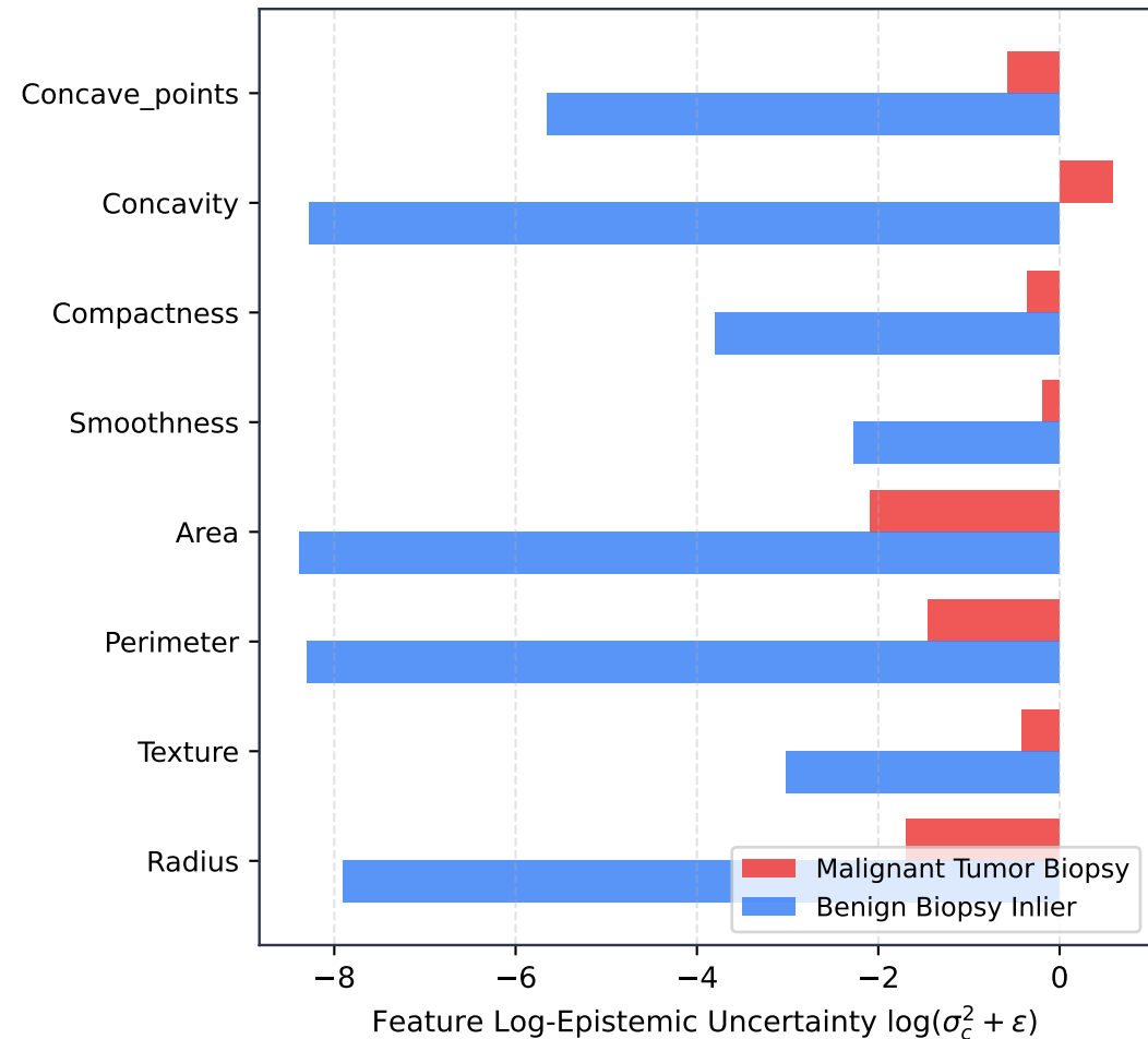
(a) WDBC Breast Cancer Attribution (AUROC = 1.0)
