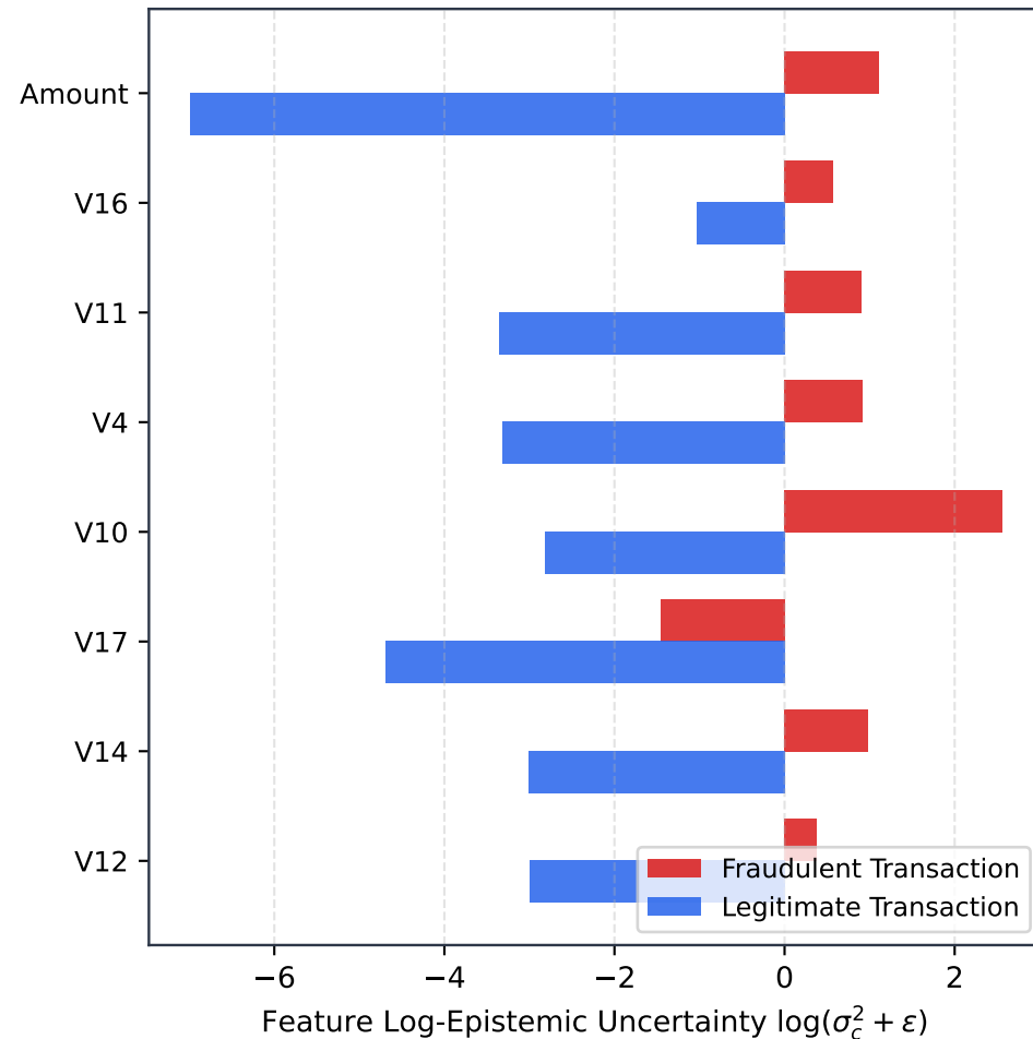
(b) Credit Card Fraud Attribution (+138% AUPRC Win)
