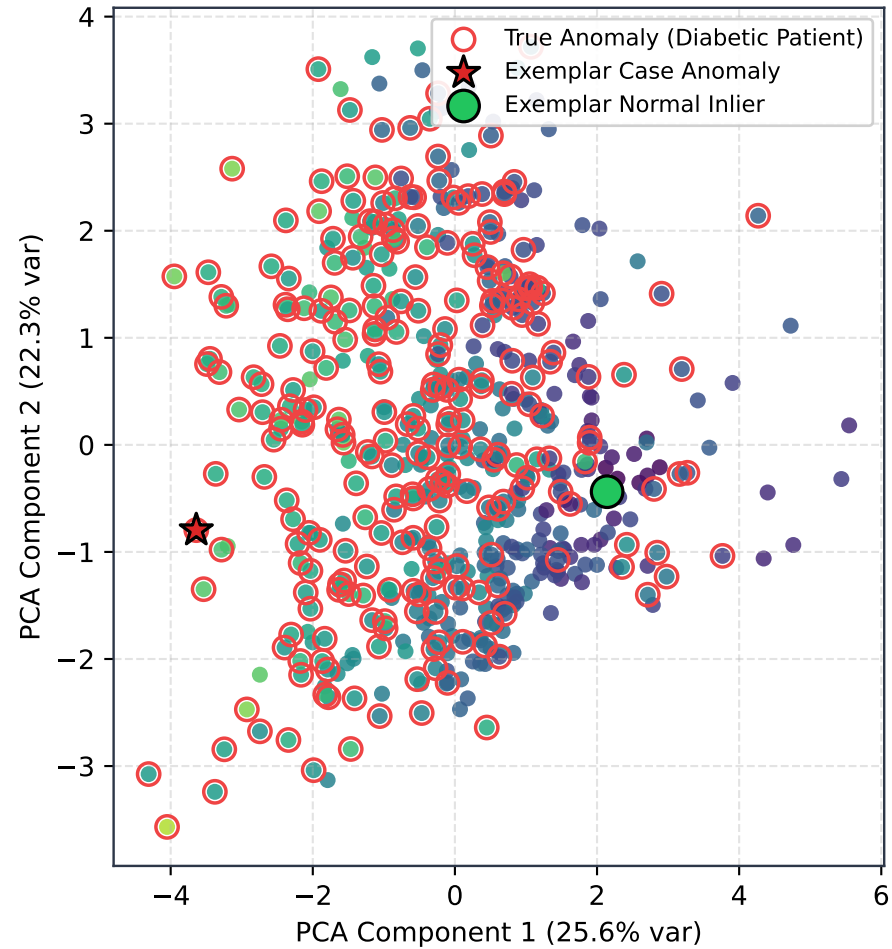
(a) Pima Diabetes Manifold & Epistemic Uncertainty
