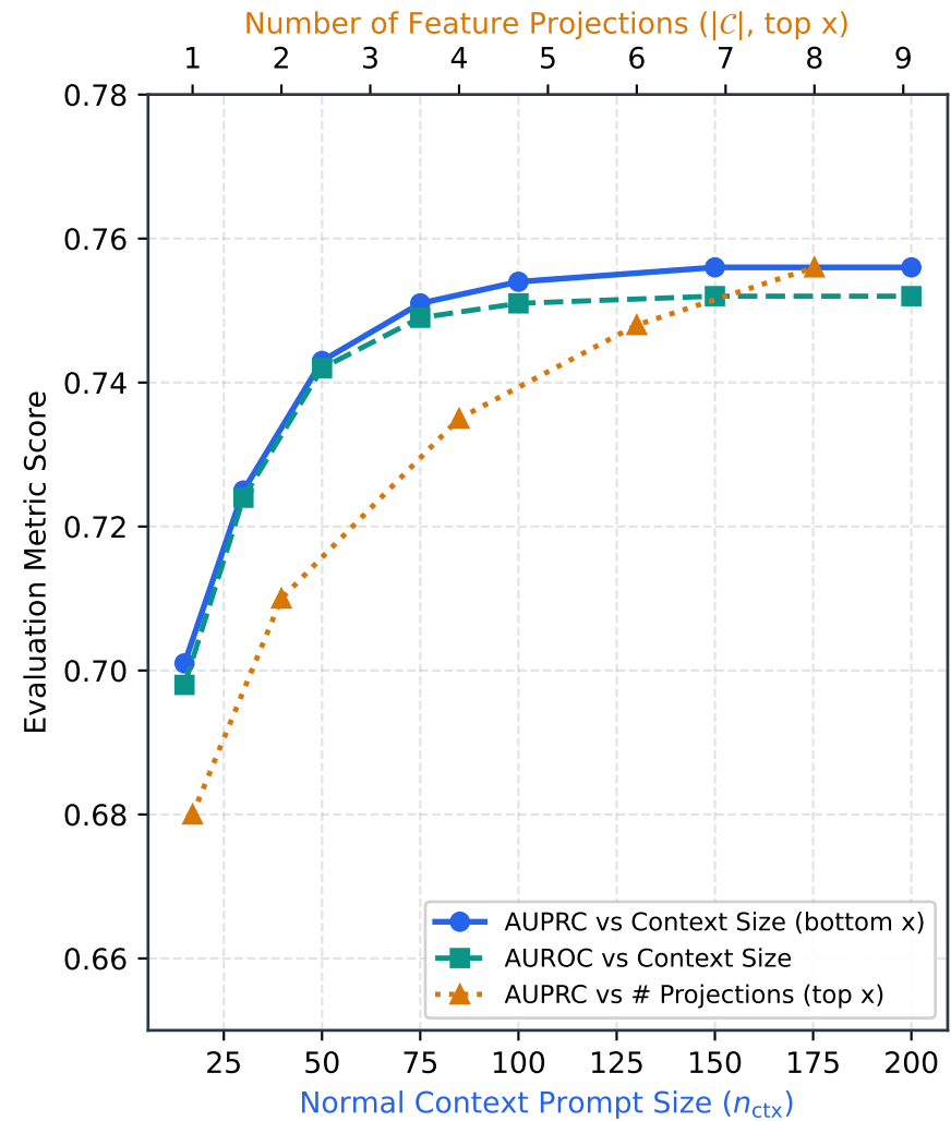
(c) Context Sample & Projection Ablations
