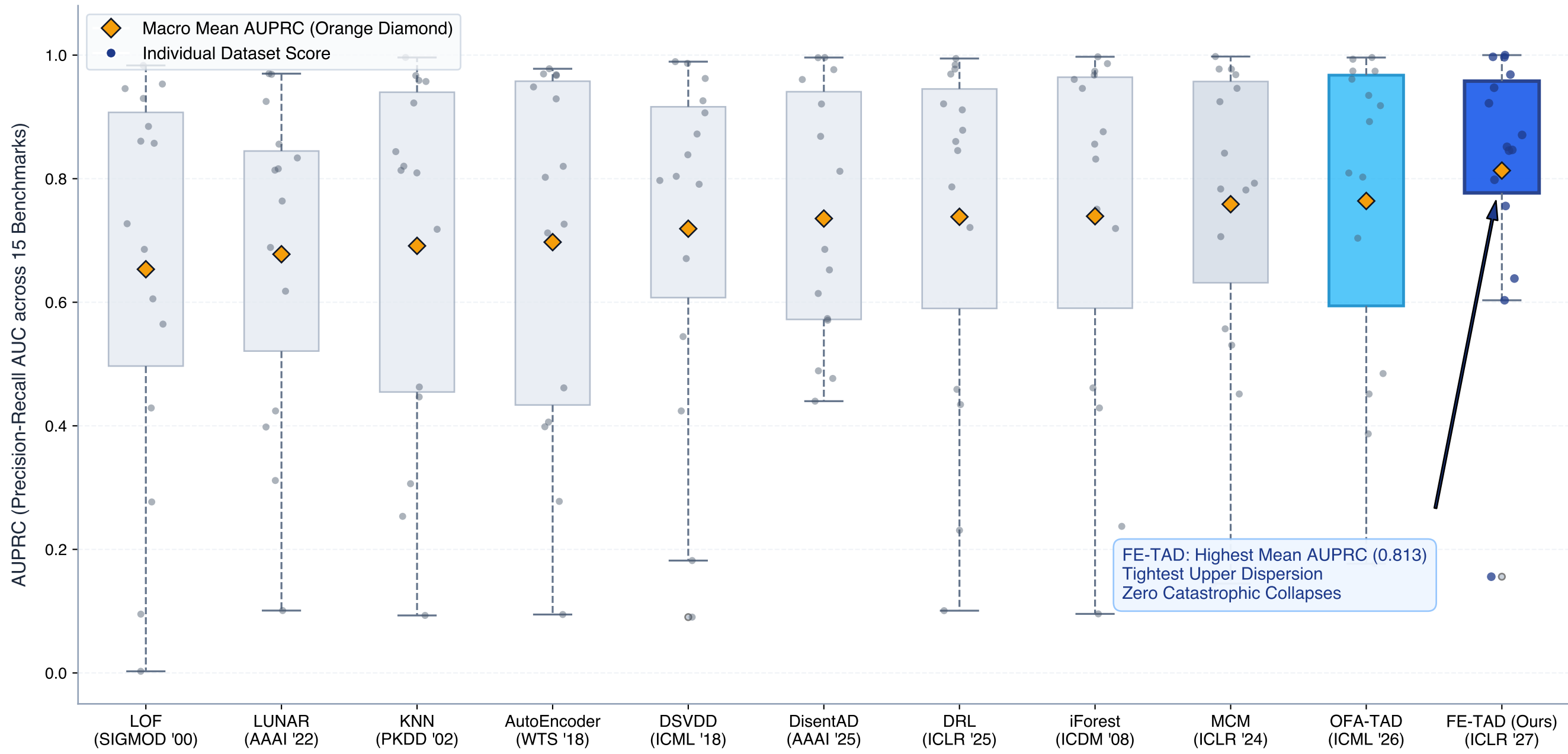
Per-Dataset AUPRC Distribution across 15 Canonical ADBench Benchmarks
