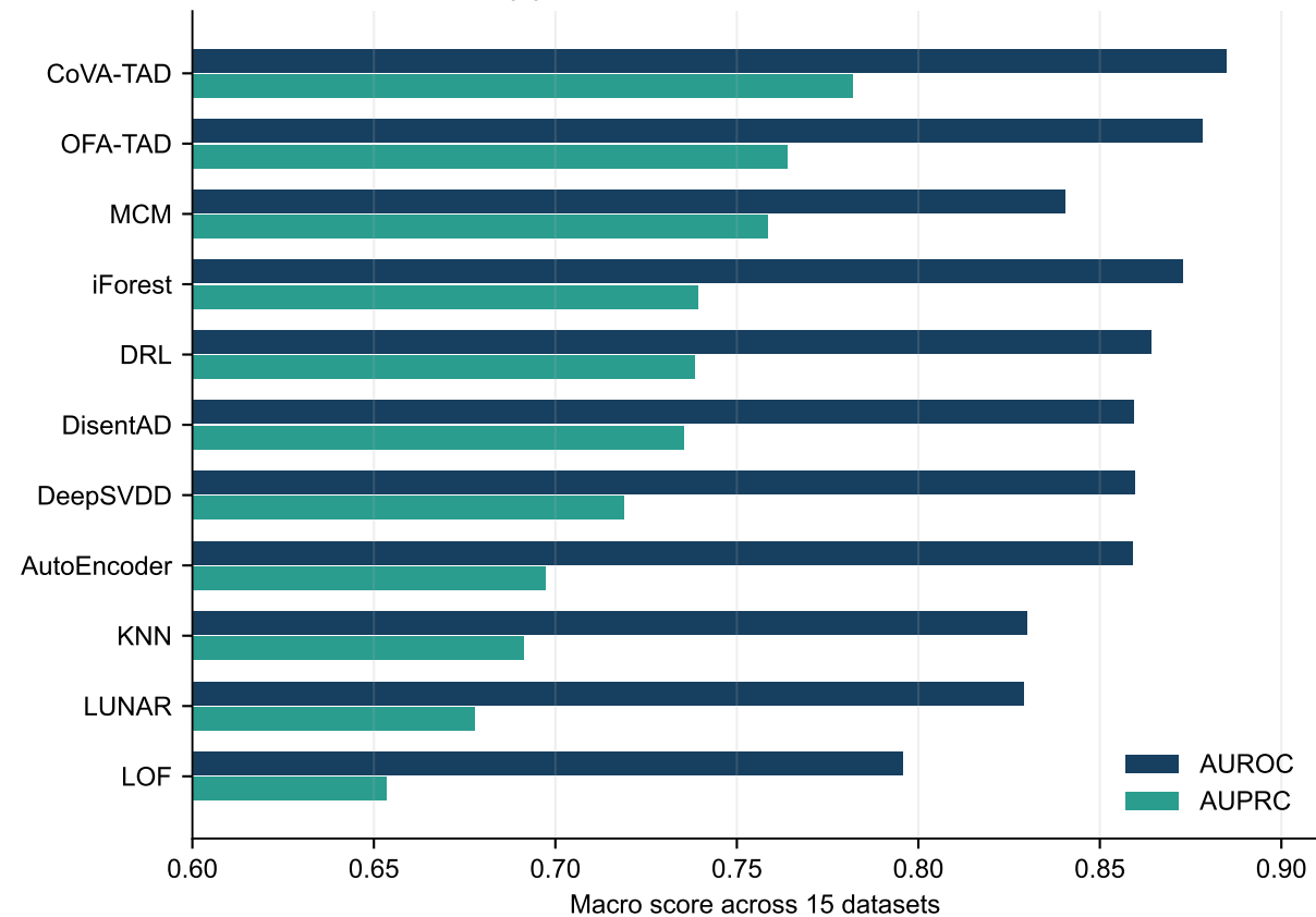
(a) All-method macro comparison
