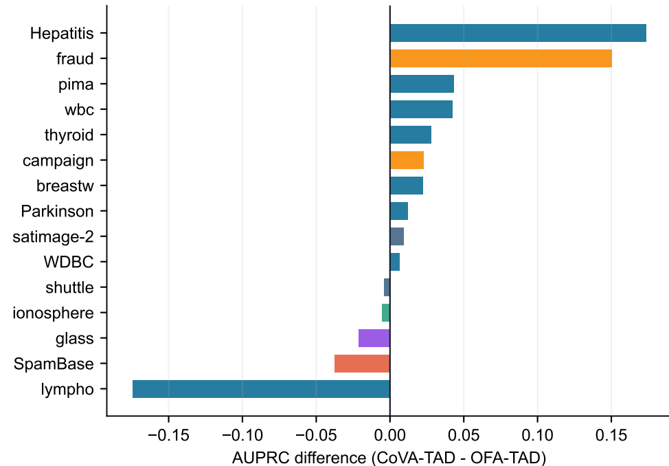
(c) Where AUPRC changes
