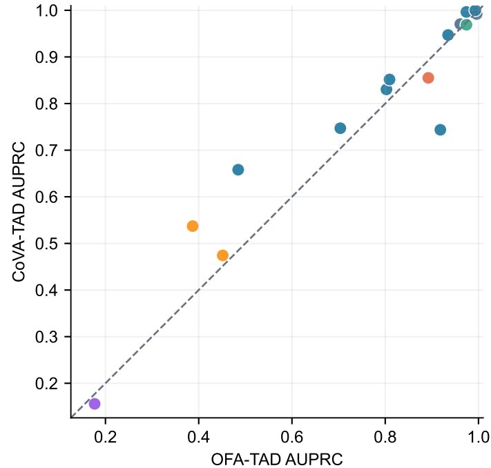
(b) AUPRC: 10/15 wins
