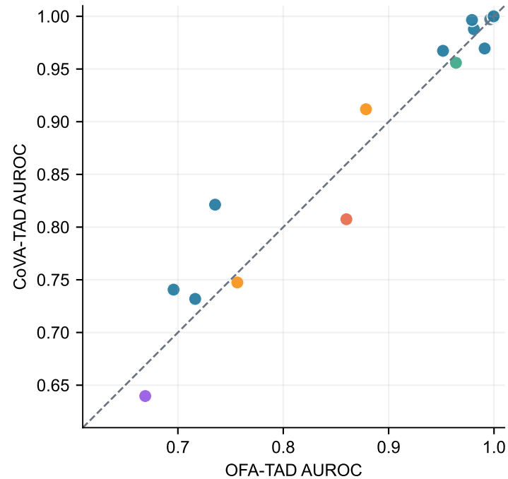
(a) AUROC: 9/15 wins
