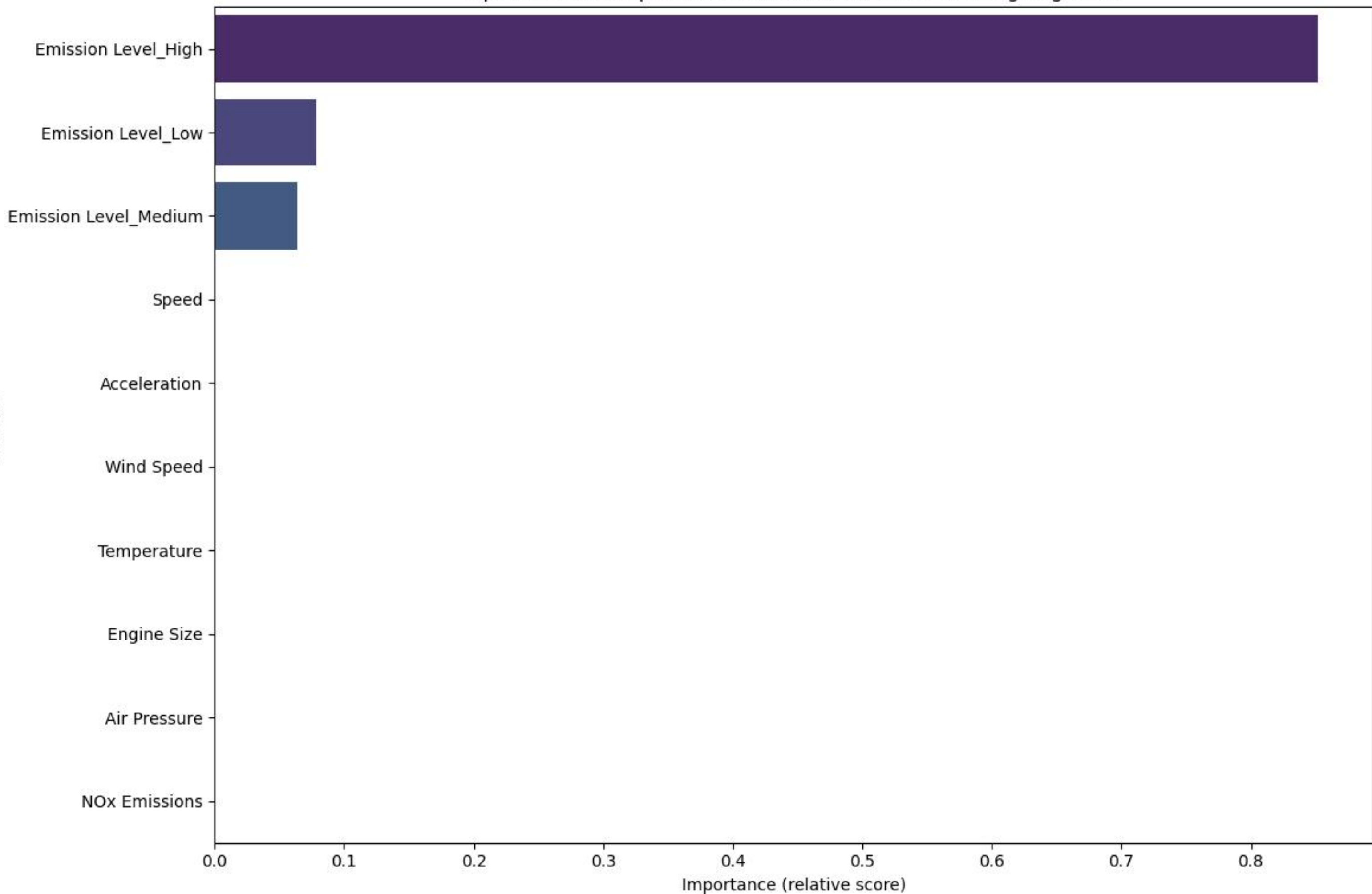
Top 10 Feature Importances for Tuned Gradient Boosting Regressor
