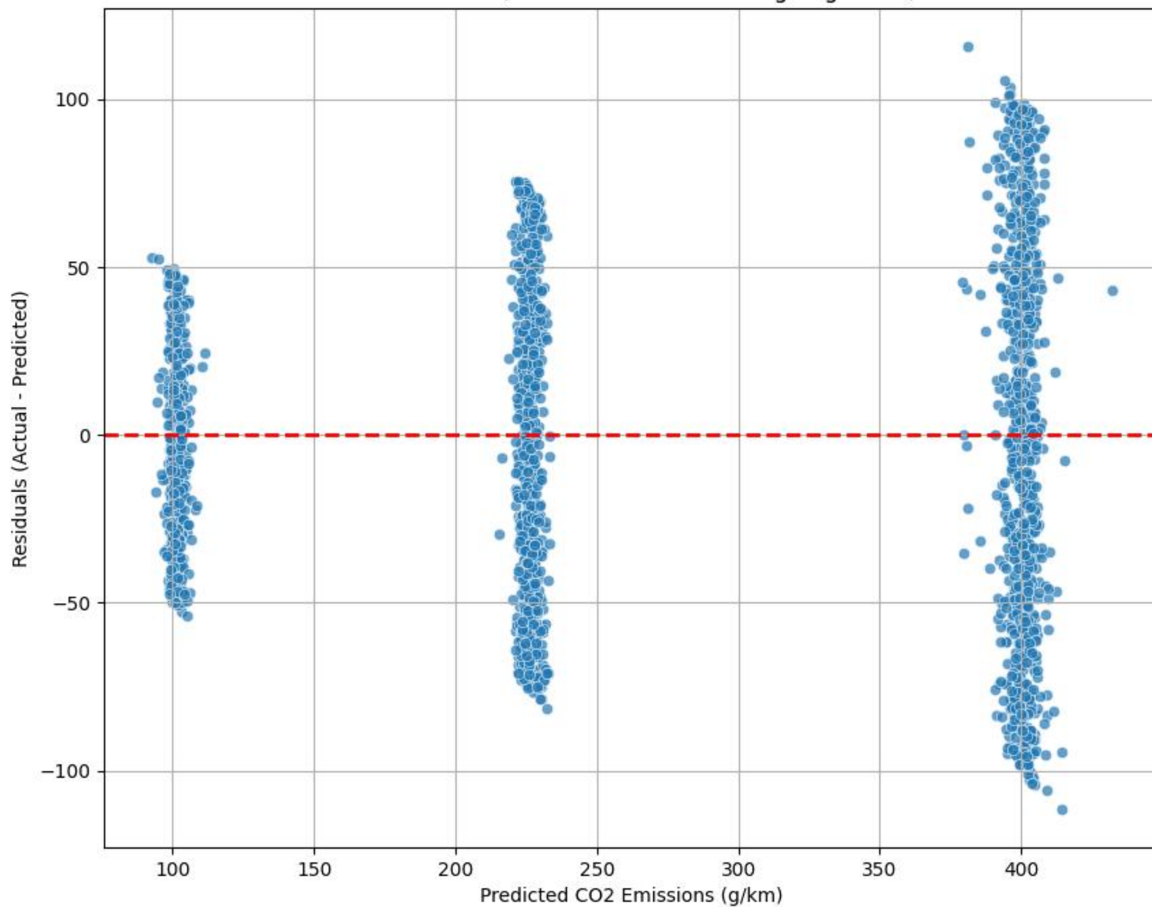
Residual Plot (Tuned Gradient Boosting Regressor)
