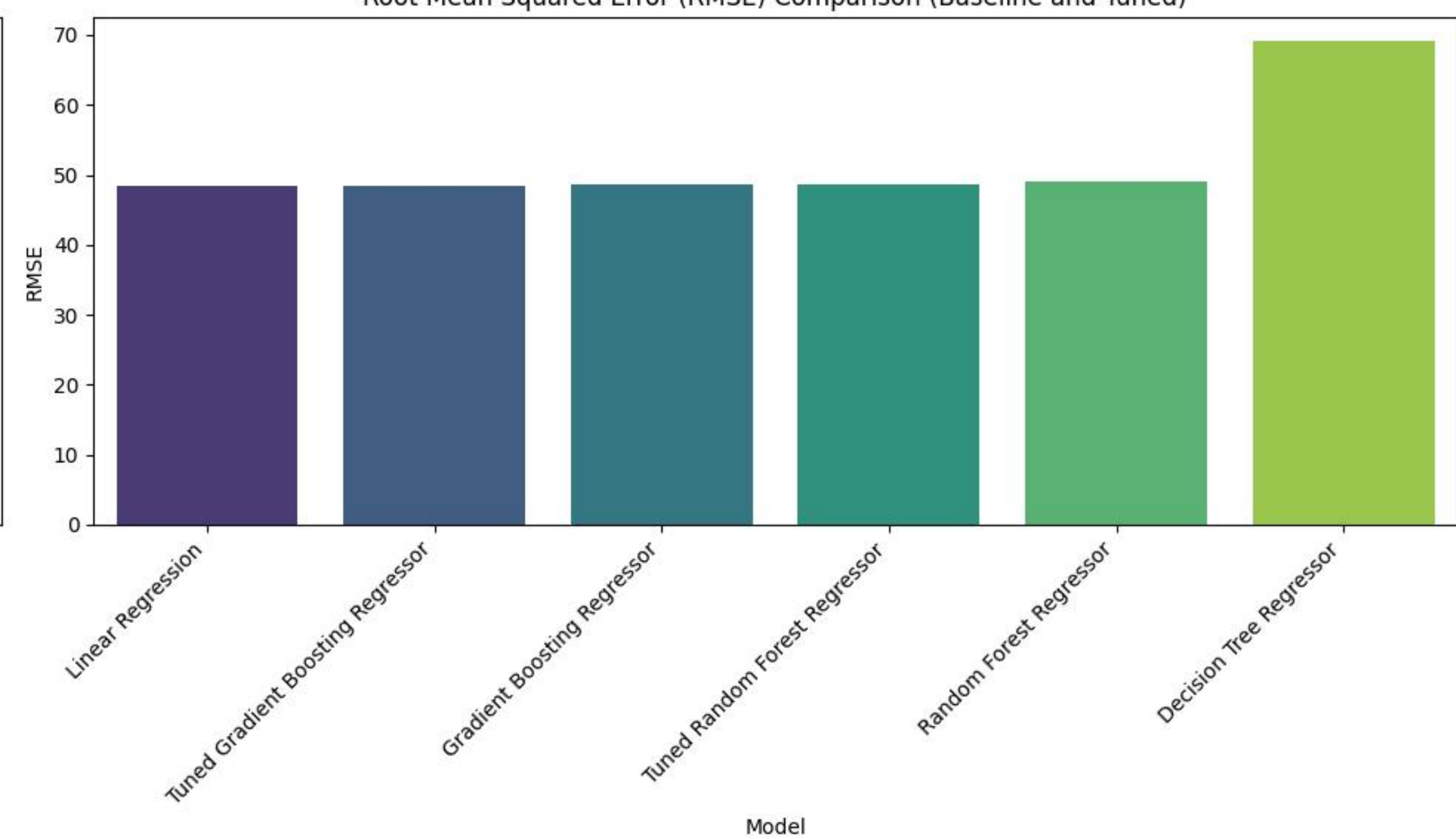
Root Mean Squared Error (RMSE) Comparison (Baseline and Tuned)
