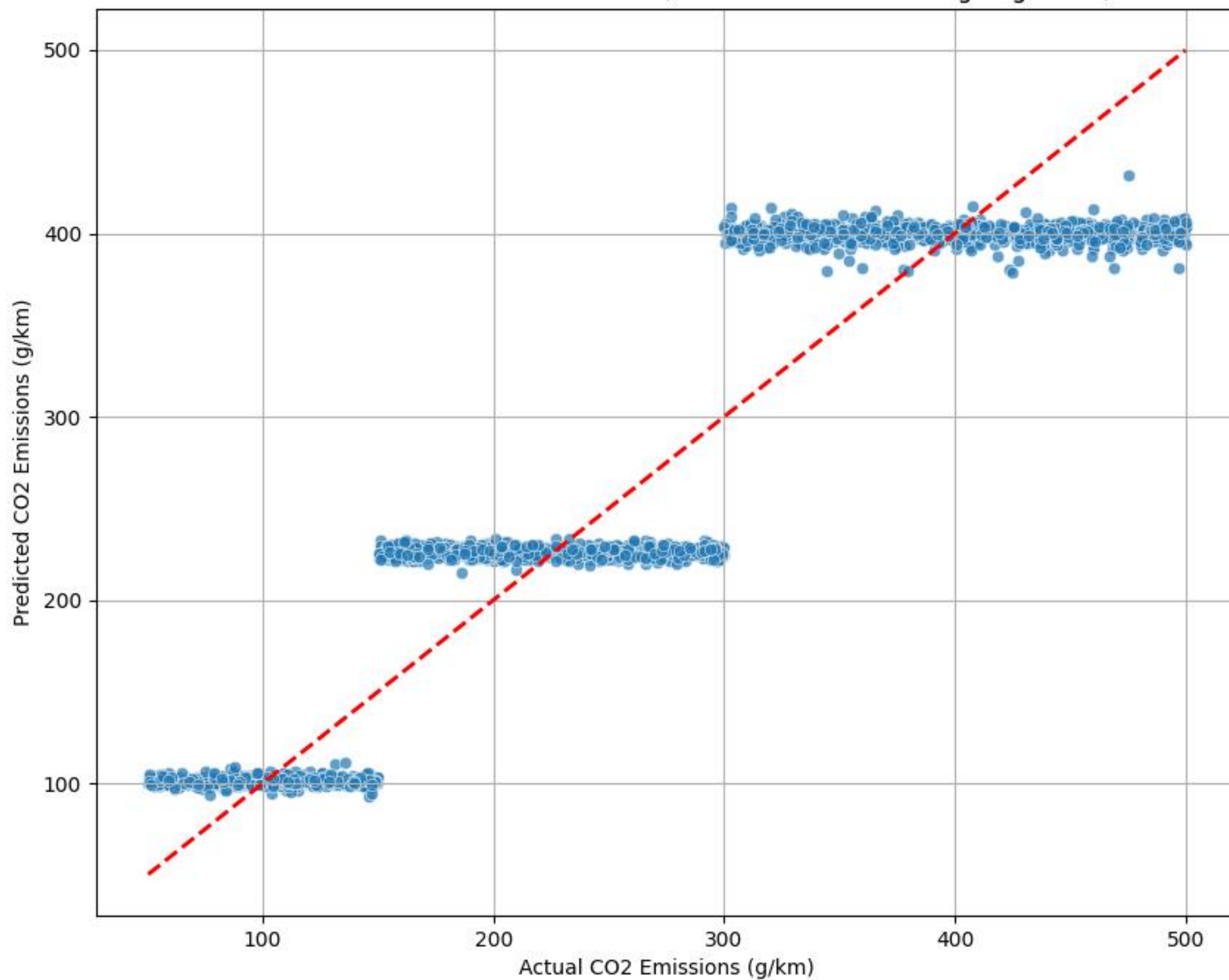
Actual vs. Predicted CO2 Emissions (Tuned Gradient Boosting Regressor)
