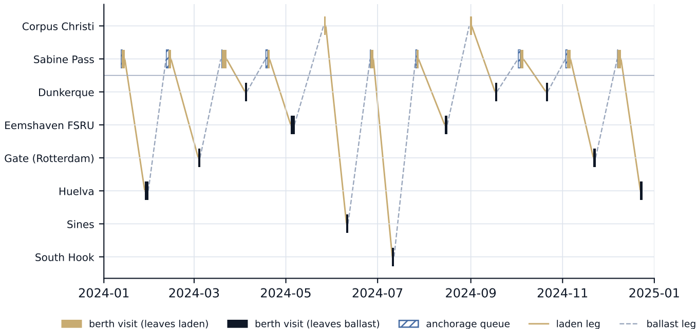
MMSI 224451000, 2024: 22 visits, 11 laden and 10 ballast legs
