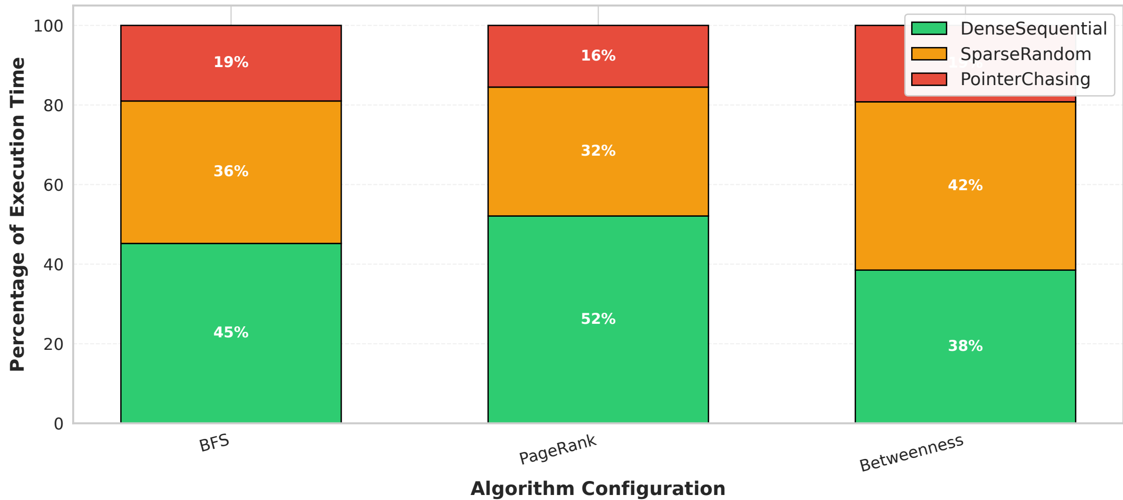
Execution Phase Distribution Across Graph Algorithms
