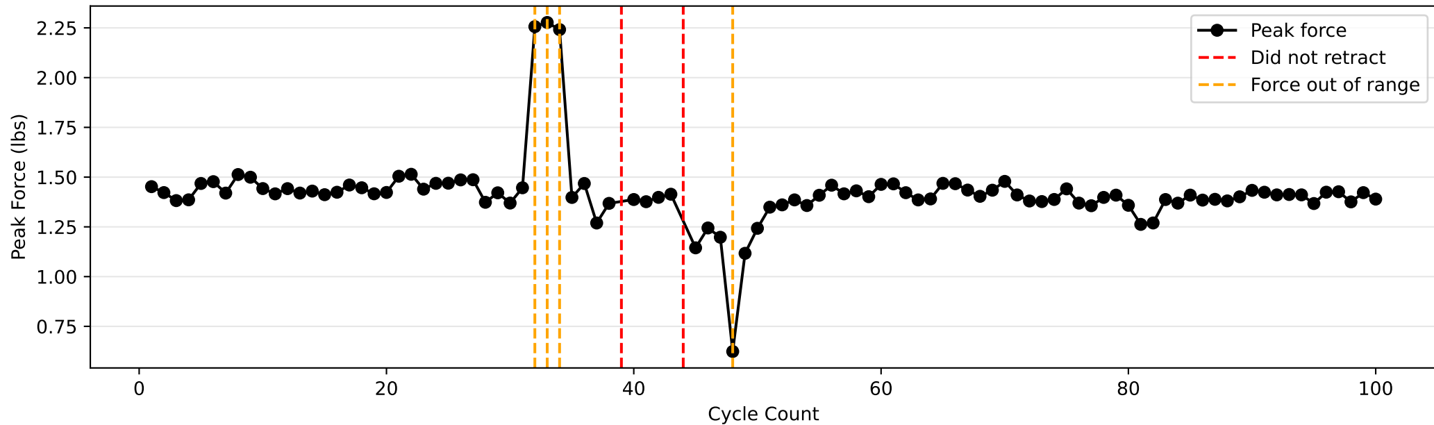
Button B: Force vs Cycle
