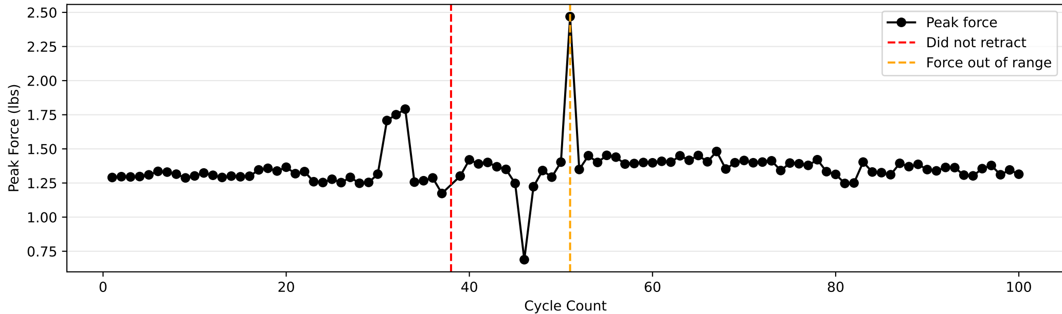
Button D: Force vs Cycle
