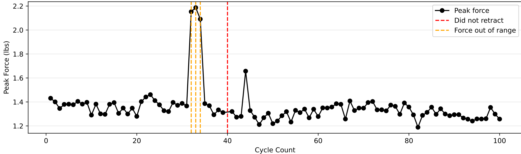
Button A: Force vs Cycle
