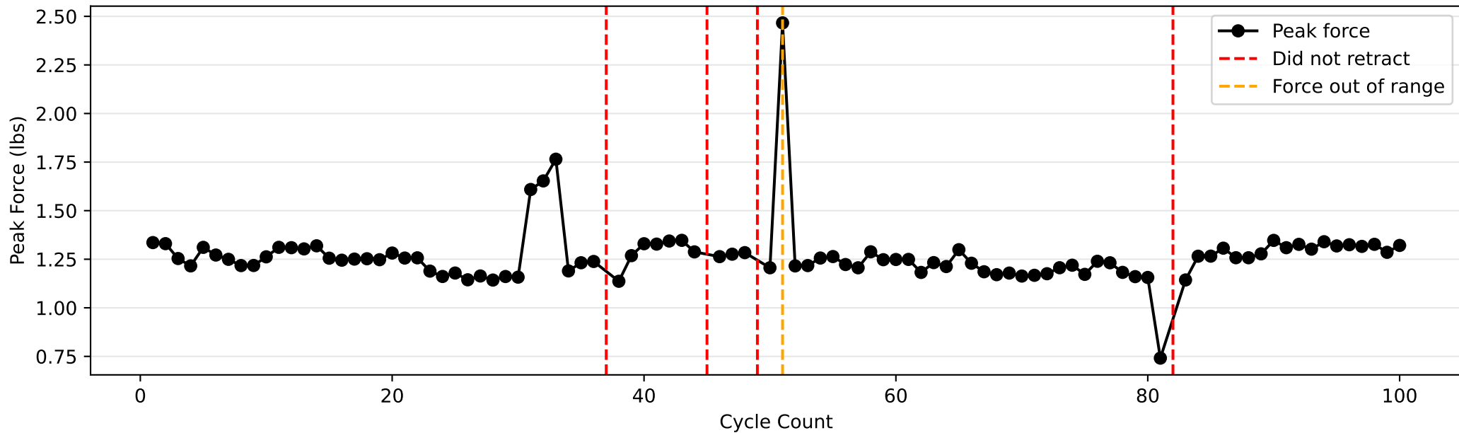
Button C: Force vs Cycle
