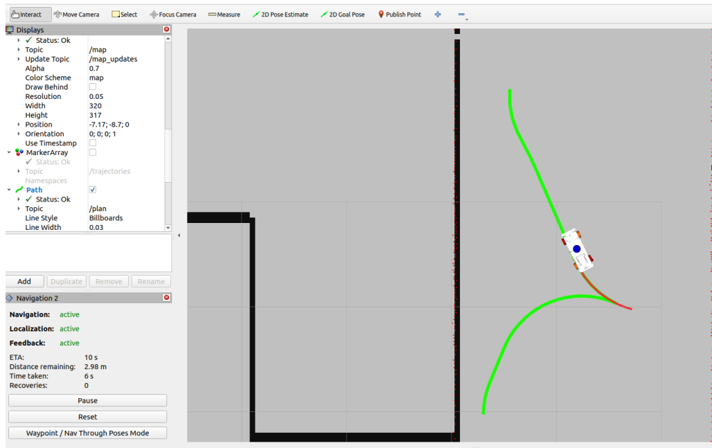
Figure 6.10: RViz during one of the simulated reversal-manoevre trials: the navigation feedback panel (left) reports the goal as still active, with ETA and distance-remaining updating live as the vehicle follows the curved approach into the reversal.
