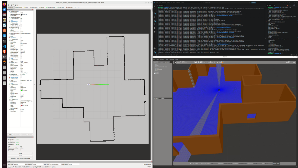
Figure 3.1: The Nav2 stack running end-to-end during this simulation bring-up: bring-up log (top right, showing each server and lifecycle manager activating in turn), RViz with the global plan and live navigation feedback panel (left) and the simulated vehicle executing the goal (bottom right).
