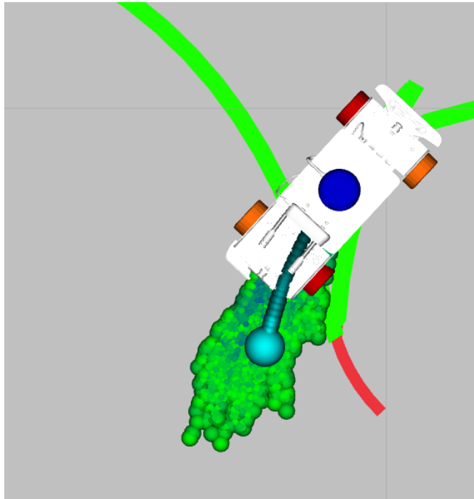
Figure 6.9: A reversal cusp during a simulated validation trial: the global plan (green) folding back on itself, with the locally-smoothed path (red) already following the corner-extended geometry of Section 6.4.5 rather than the original sharp vertex.
