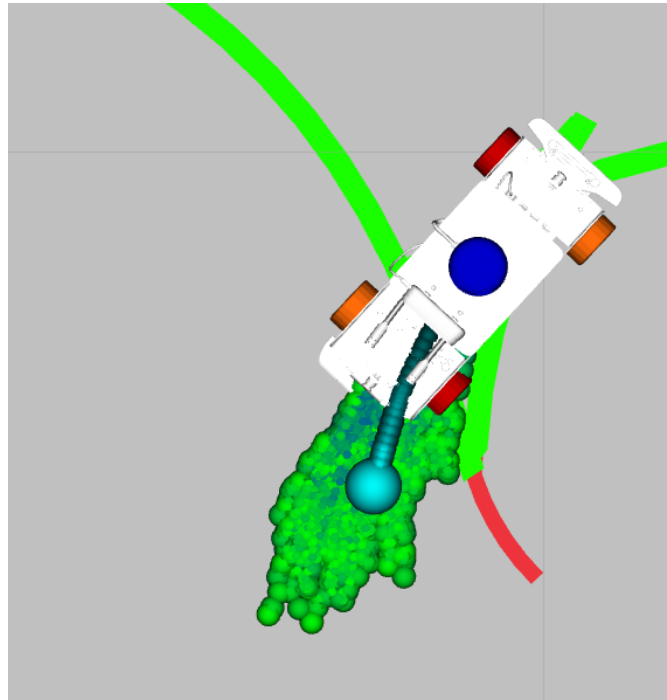
Figure 6.8: A reversal cusp during a simulated validation trial: the global plan (green) folding back on itself, with the locally-smoothed path (red) already following the corner-extended geometry of Section 6.4.5 rather than the original sharp vertex.
