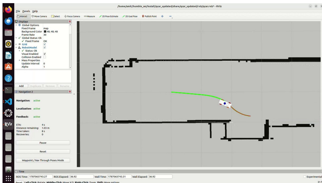
Figure 6.2: RViz during the right-turn trial: the global plan (green) curves the vehicle out of the corridor junction towards the goal, with the navigation feedback panel (left) reporting distance remaining and elapsed time as the turn is executed.
