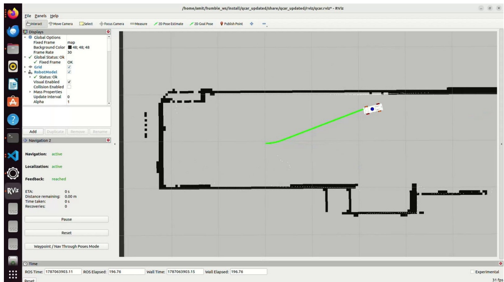
Figure 6.4: RViz during the left-turn trial: the navigation feedback panel reports Feedback: reached with zero distance remaining at the end of the curved approach.
