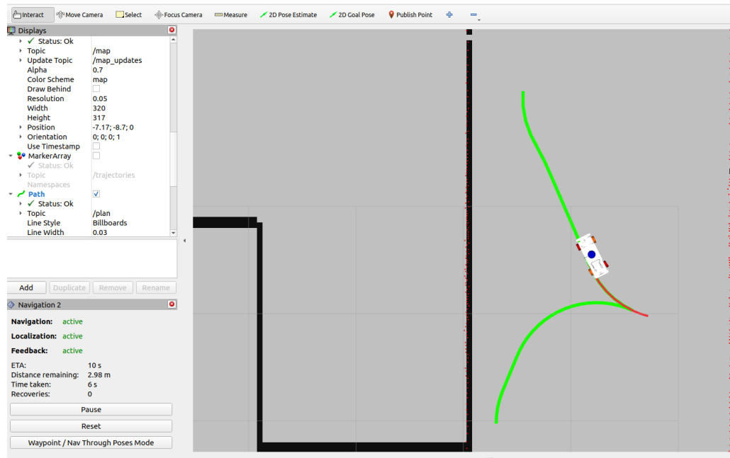
Figure 6.9: RViz during one of the simulated reversal-manoevre trials: the navigation feedback panel (left) reports the goal as still active, with ETA and distance-remaining updating live as the vehicle follows the curved approach into the reversal.
