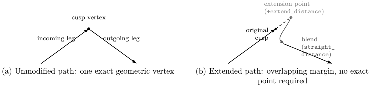
Figure 6.7: The corner-extension mechanism of Listing 6.3. (a) The planner’s raw output meets the incoming and outgoing legs at one precise vertex, which MPPI’s inversion-tolerance gate must satisfy exactly. (b) The smoother pushes the cusp outward along the incoming leg’s own heading before blending back to the outgoing leg, so the two legs deliberately overlap – trading one brittle exact target for a geometric margin the controller can negotiate.
