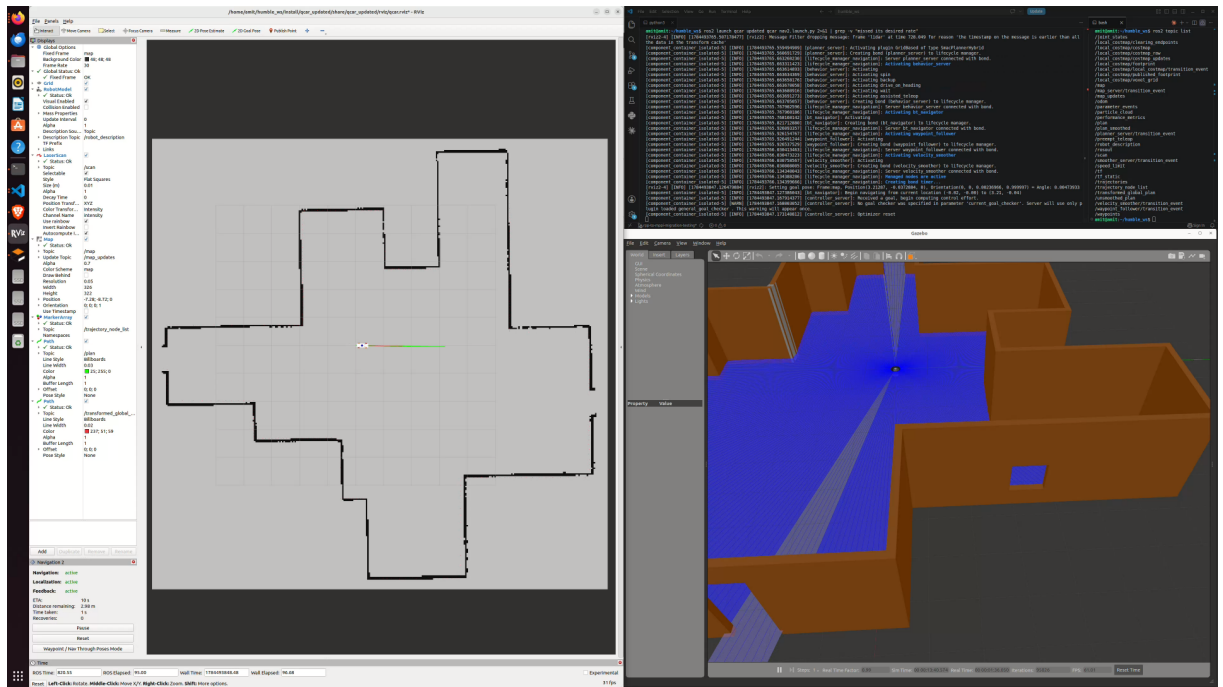
Figure 6.3: The Nav2 stack running end-to-end on the simulation branch of the same launch configuration: bring-up log (top right, showing each server and lifecycle manager activating in turn), RViz with the global plan and live navigation feedback panel (left) and the simulated vehicle executing the goal (bottom right).
