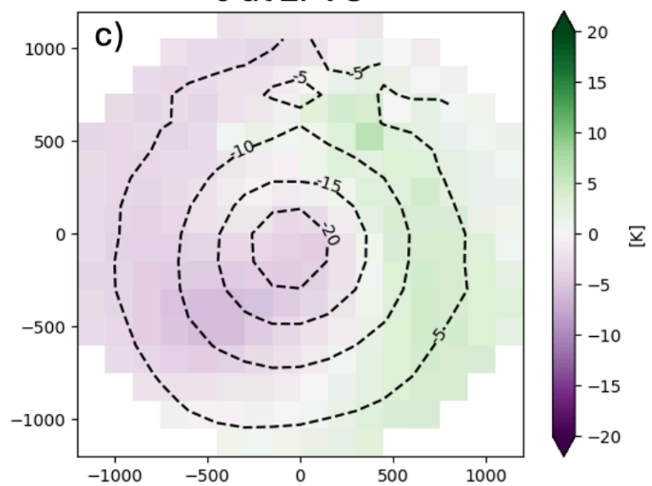
\theta at 2PVU
