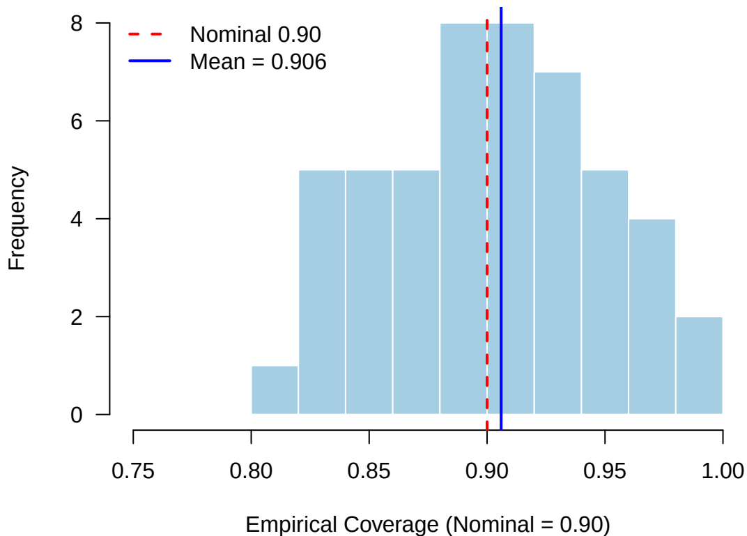
Figure 3: Empirical Coverage Across 50 Splits
