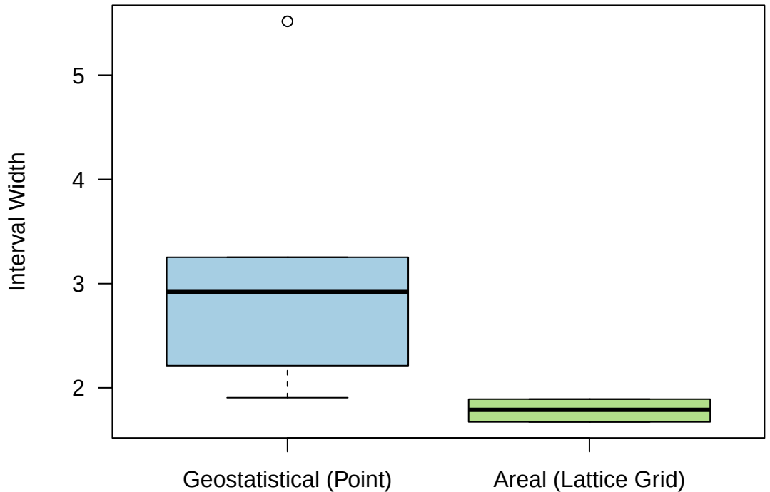
Figure 7: Interval Width Distribution
