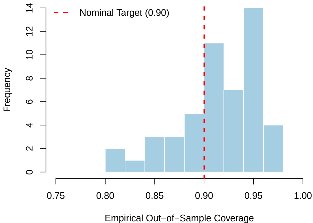
Figure 3: Empirical Coverage Across 50 Random Splits
