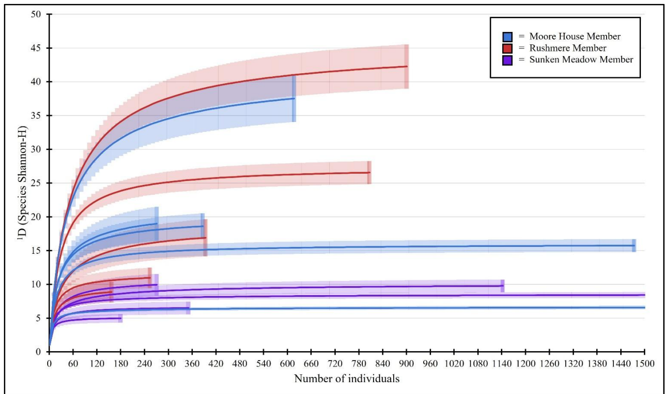
FIG. S3. – Sample-size-based diversity accumulation curves for {}^1D (Shannon-H, \pm 95% CI) at the species level. Rarefaction was calculated at intervals of 10 individuals, and curves end at total sample size or at 1500 individuals for large samples.
