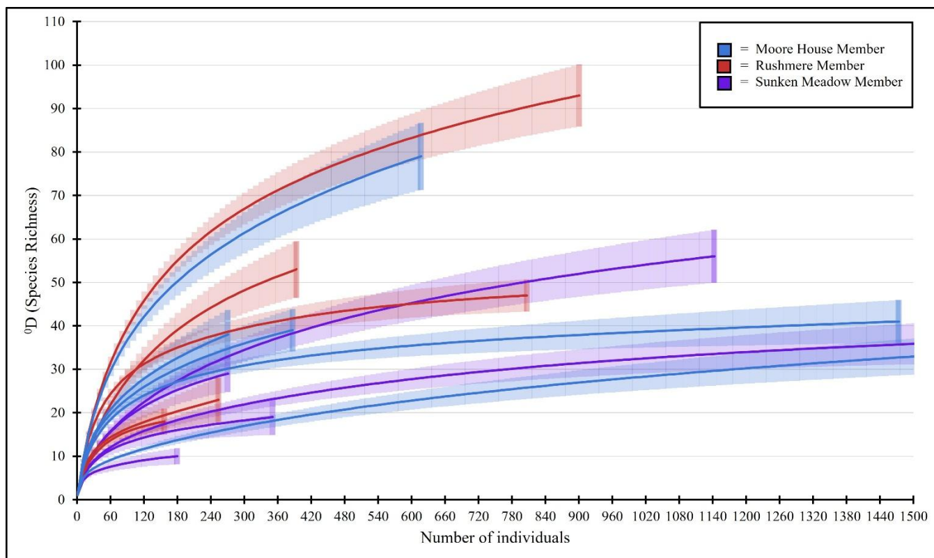
FIG. S2. – Hill numbers rarefaction curves for {}^0D (richness, \pm 95\% CI) at the species level. Rarefaction was calculated at intervals of 10 individuals, and curves end at total sample size or at 1500 individuals for large samples.
