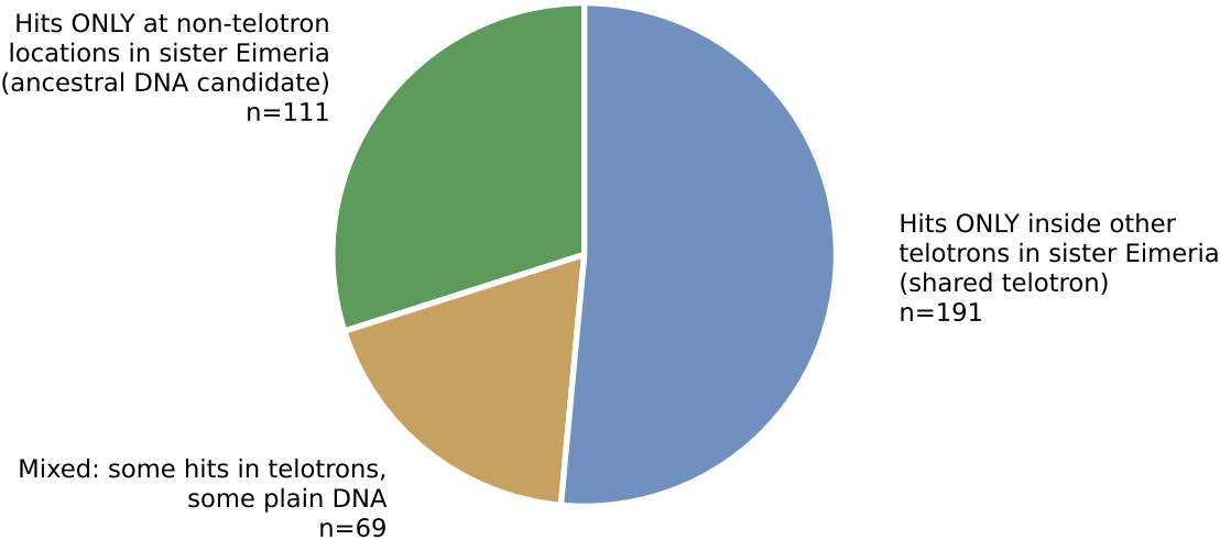
B. Where do cross-Eimeria hits land? (n=371 linkers with Eimeria hits)
