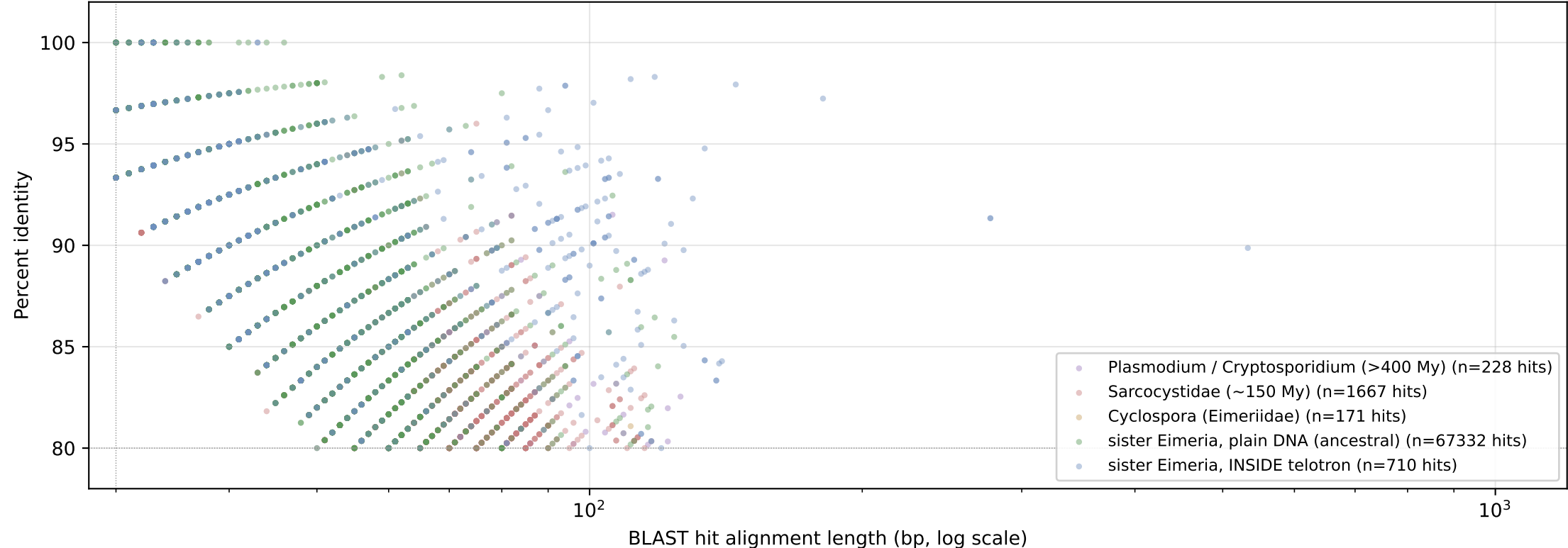
C. BLAST hit length vs identity, colored by lineage class
