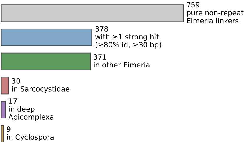
A. Linker→Apicomplexa BLAST aggregate
