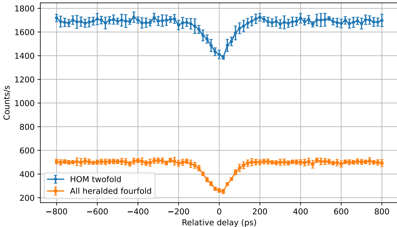
HOM twofold and heralded fourfold counts
