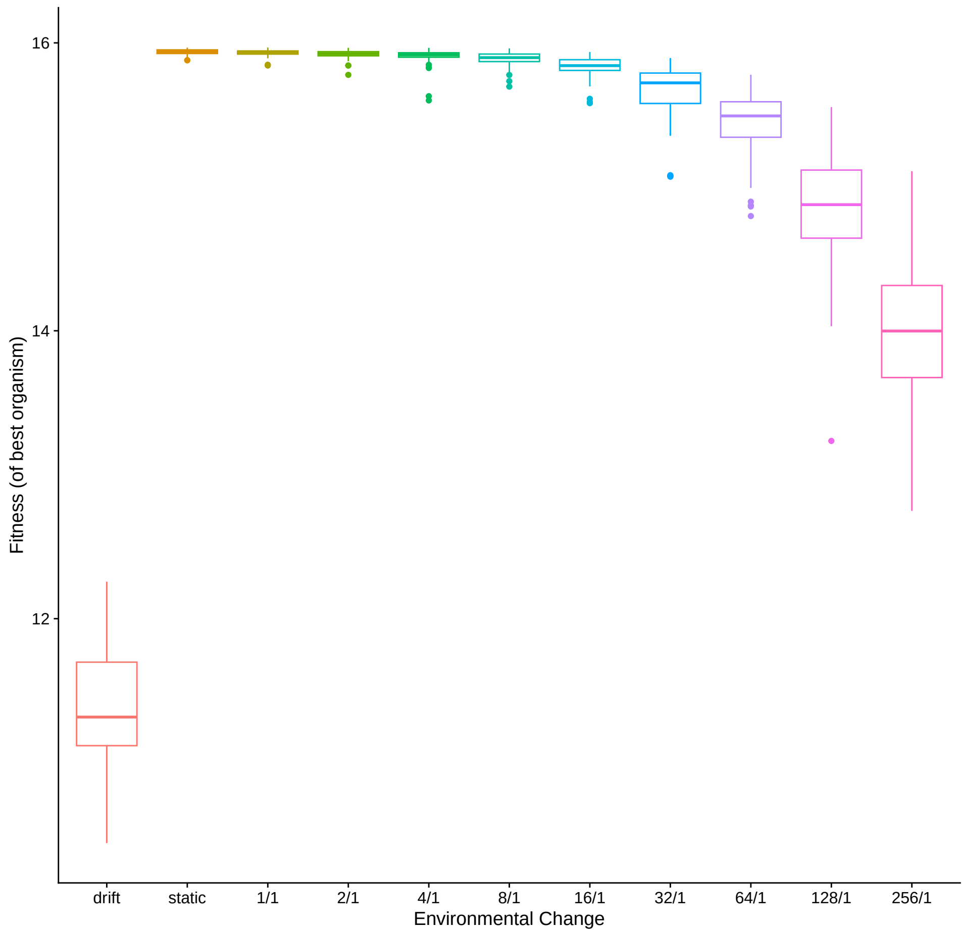
NK Fitness Model
