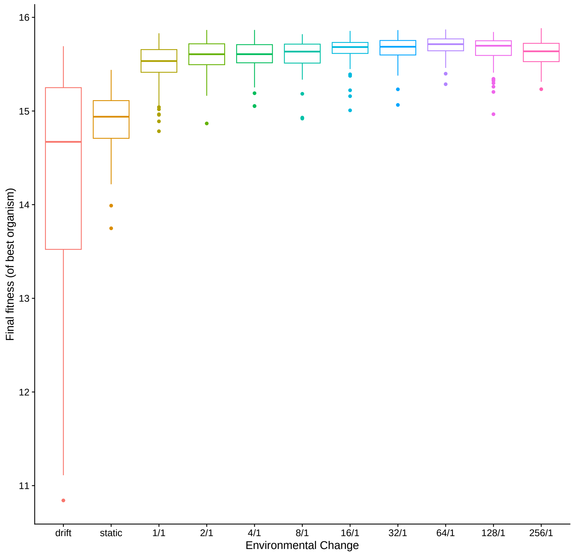
NK Fitness Model – Second experiment phase
