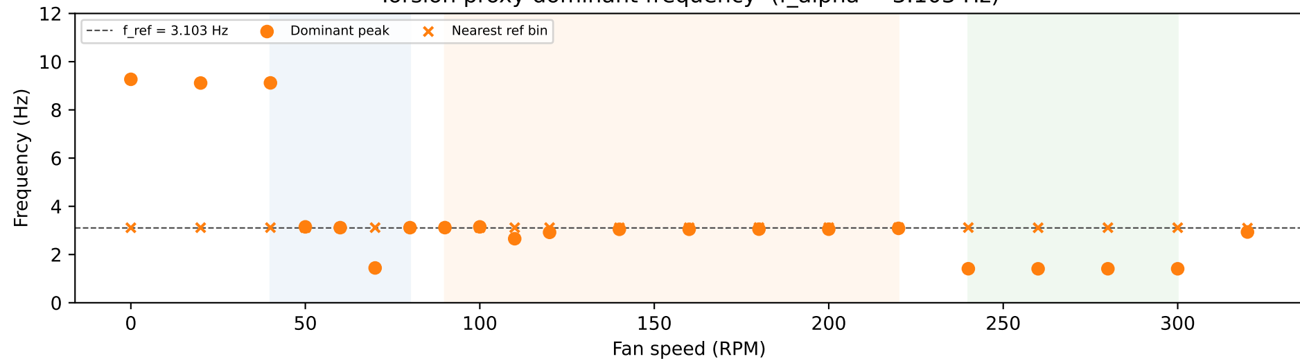
Torsion proxy dominant frequency ( f_{\alpha} = 3.103 Hz)
