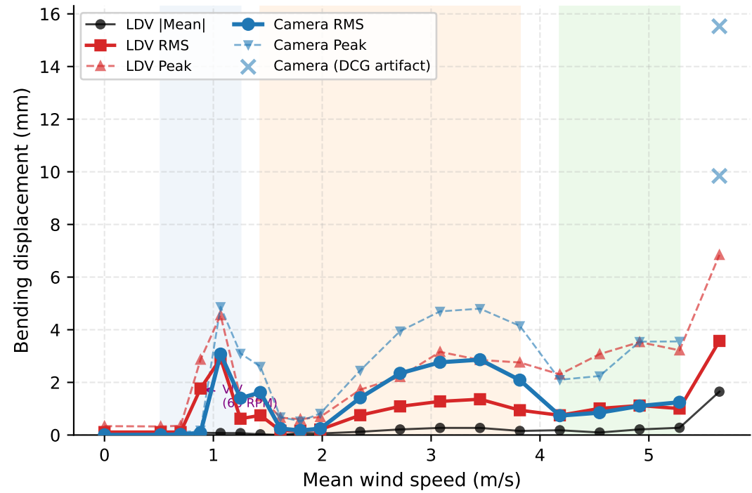
Bending — All 20 conditions
