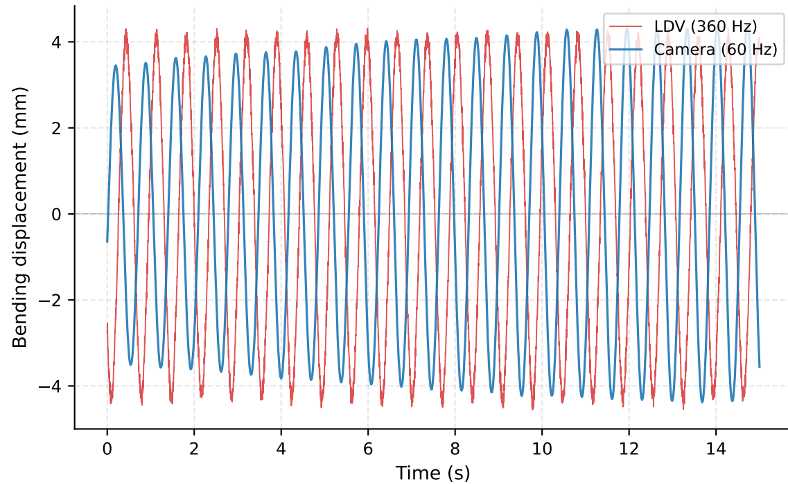
Bending VIV (70 RPM, U^*_b=1.86 ) | Bending
