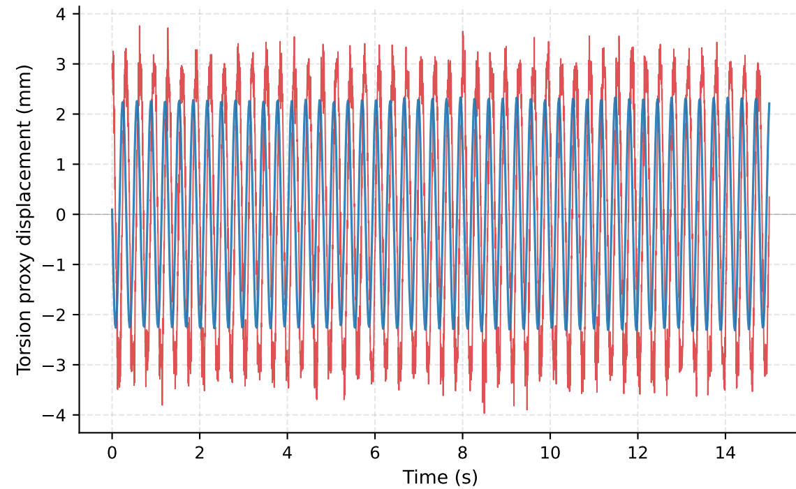
Torsional VIV (90 RPM, U^*_b=2.50 ) | Torsion proxy
