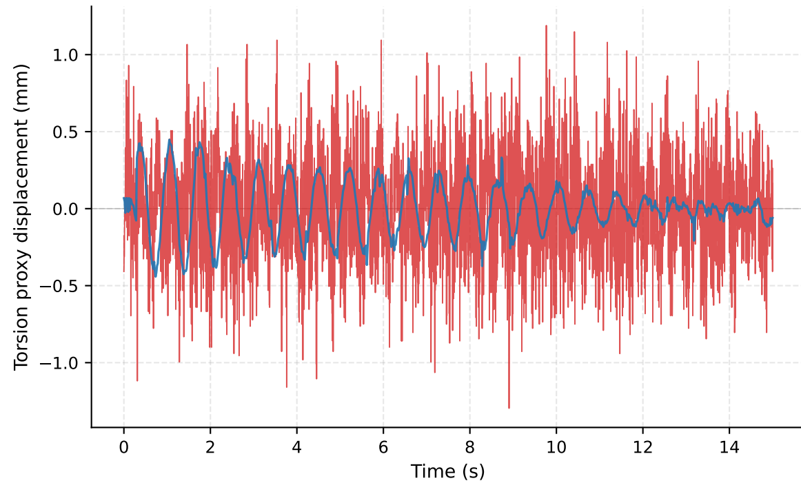
Bending VIV (70 RPM, U^*_b=1.86 ) | Torsion proxy
