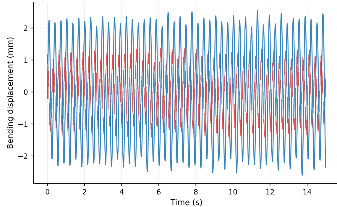
Torsional VIV (90 RPM, U^*_b=2.50 ) | Bending
