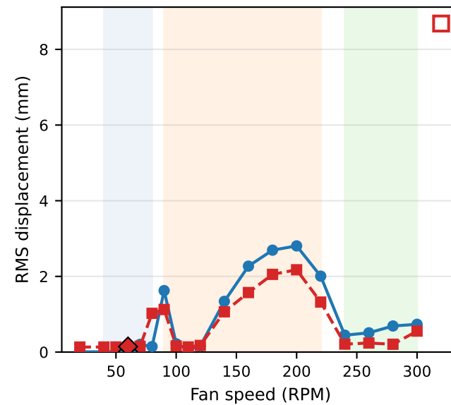
(e) Torsion RMS
