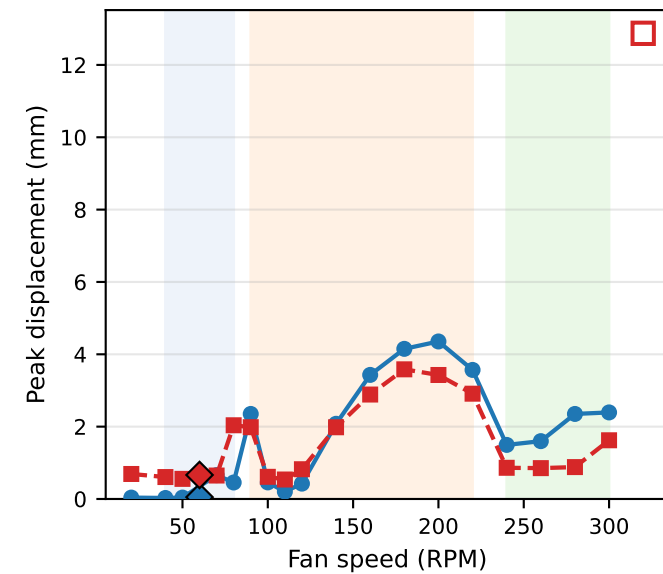
(f) Torsion Peak
