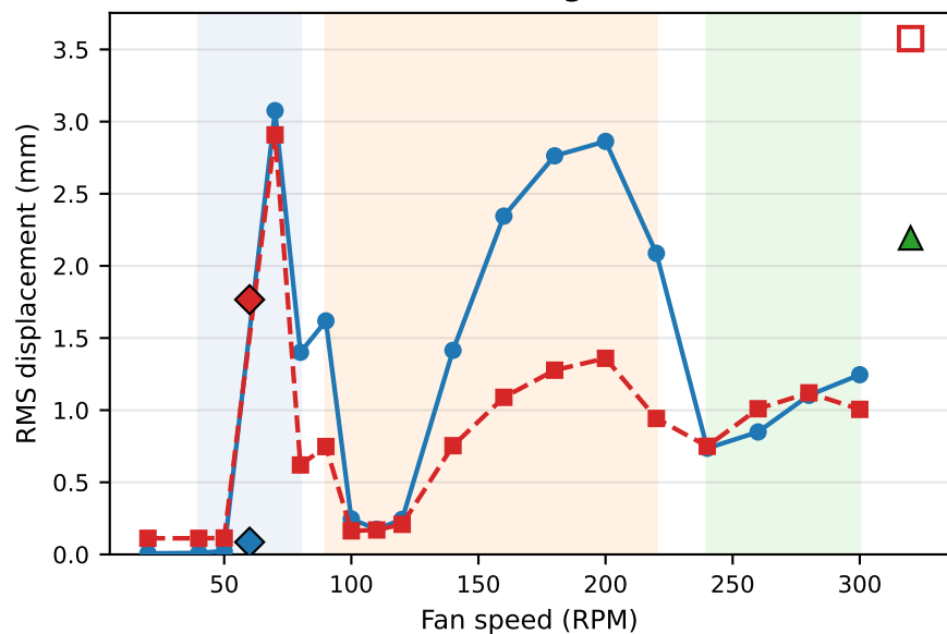
(a) Bending RMS
