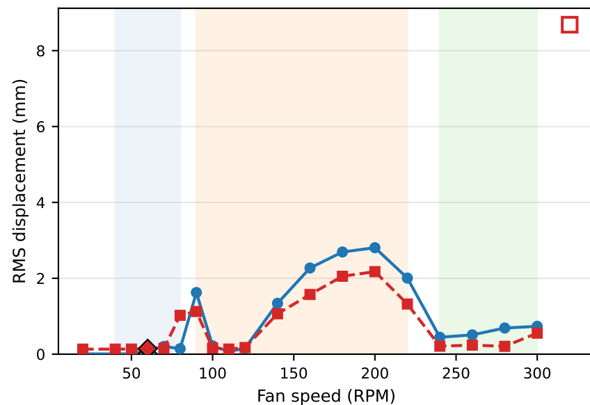
(b) Torsion RMS
