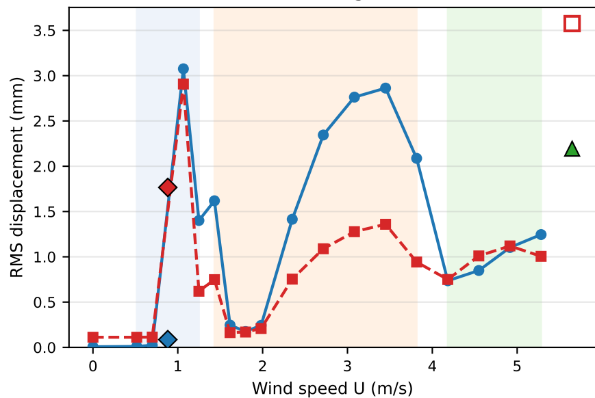
(c) Bending RMS
