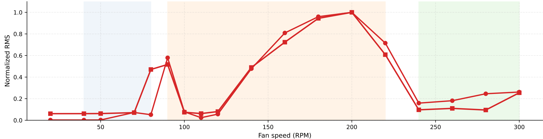
Normalized torsion-proxy RMS (stable conditions)
