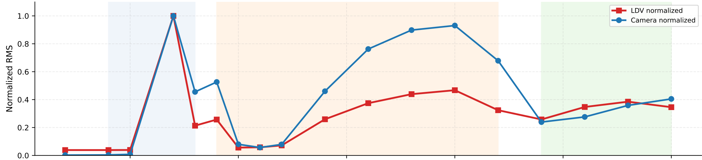
Normalized torsion-proxy RMS (stable conditions)
