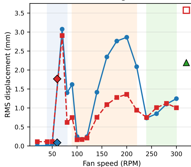
(b) Bending RMS
