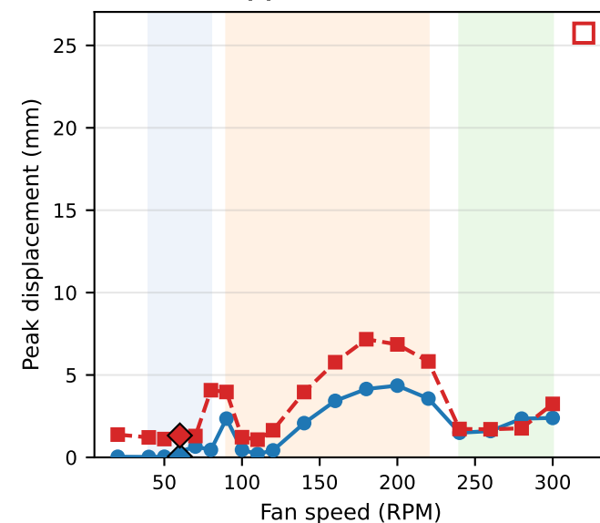
(f) Torsion Peak
