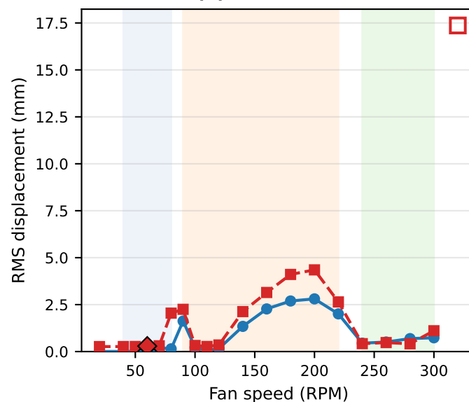
(e) Torsion RMS
