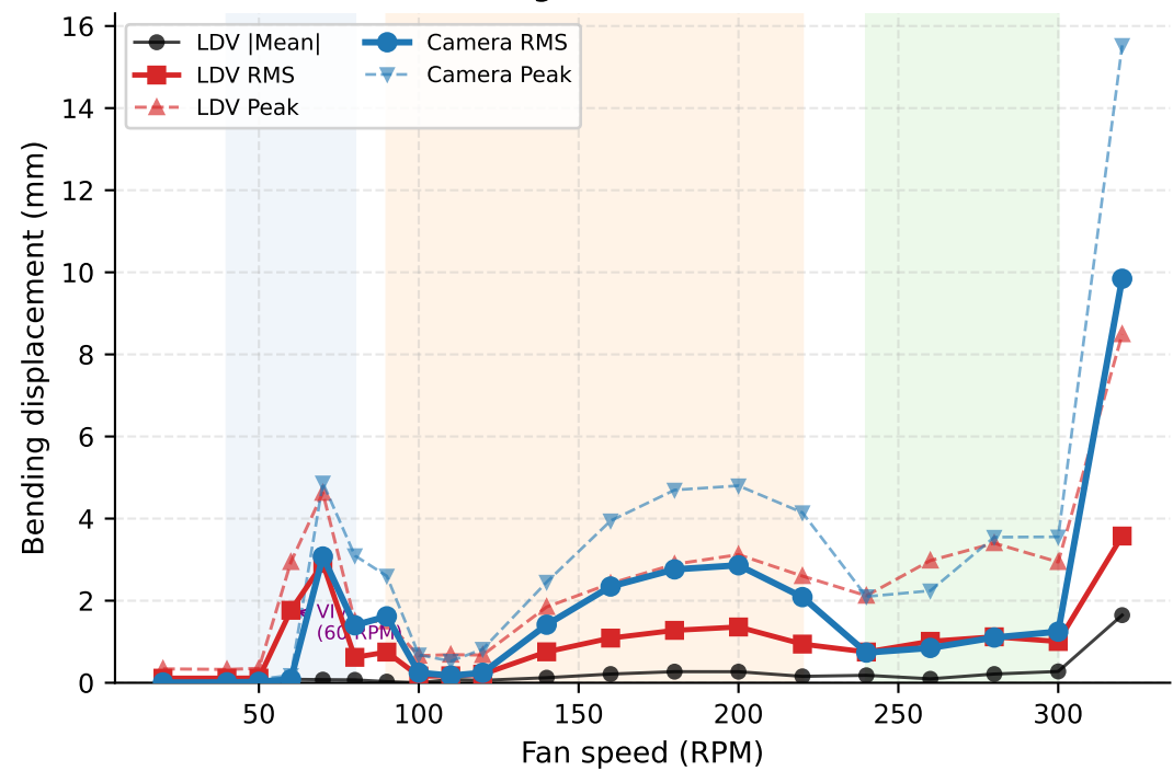
Bending — All 20 conditions
