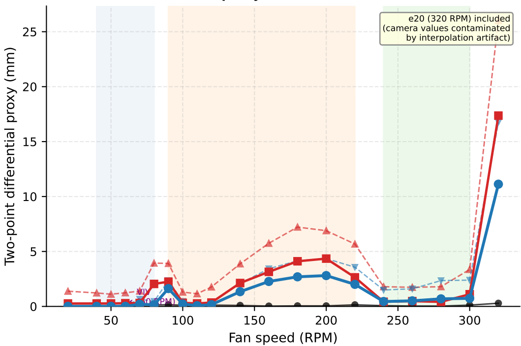
Torsion proxy — All 20 conditions
