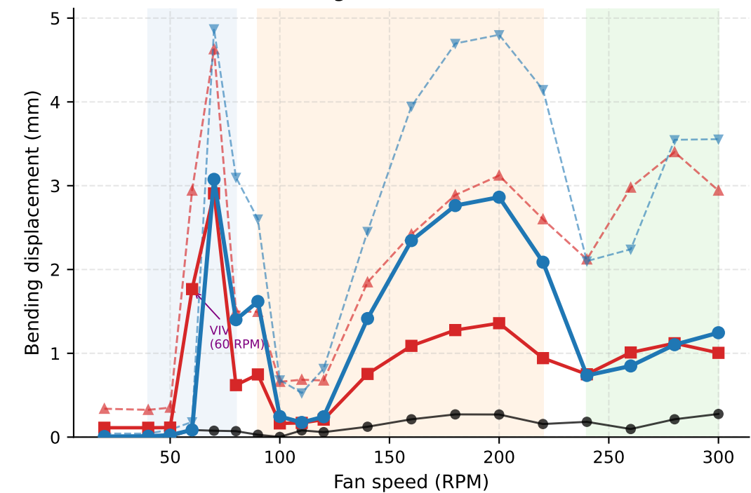
Bending — e20 DCG-excluded
