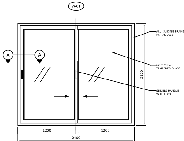
ELEVATION - W-01 (VIEWED FROM OUTSIDE)
