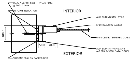
SECTION A-A - TYPICAL JAMB
