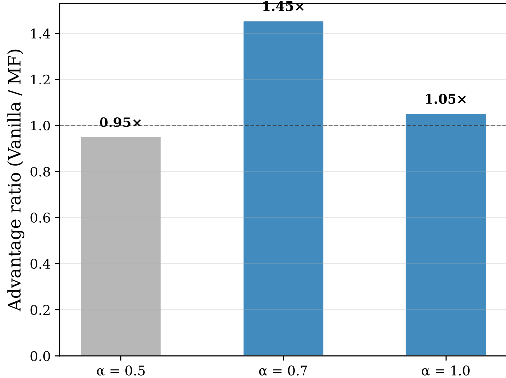
(b) MF advantage factor
