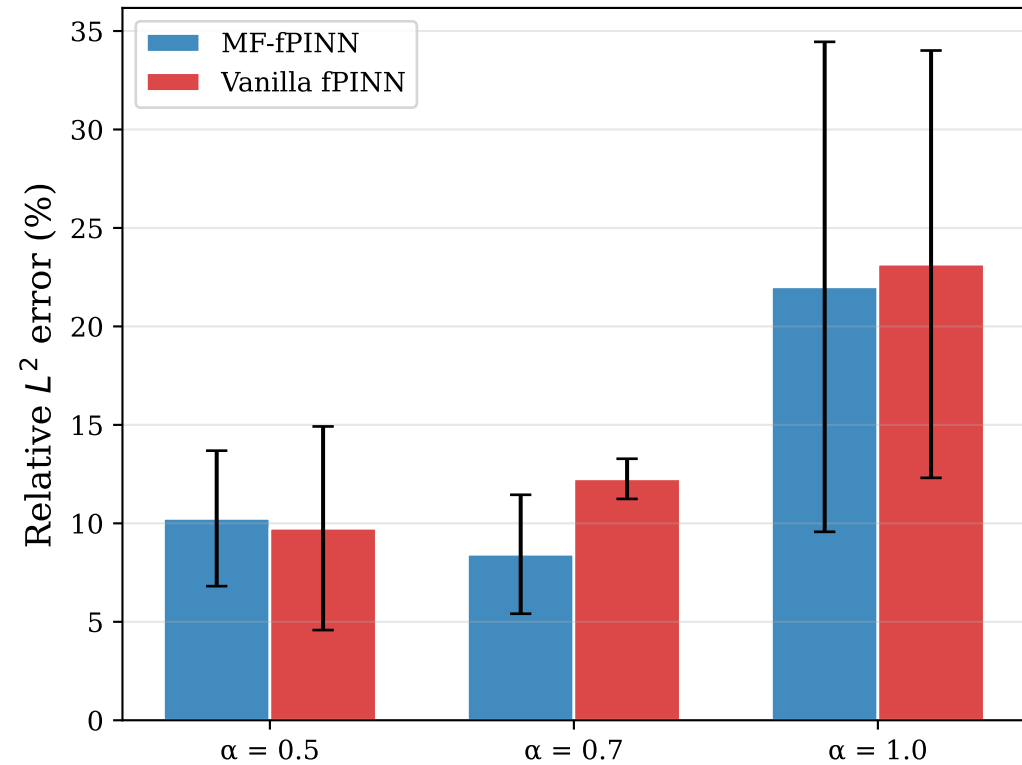
(a) MF vs Vanilla at N_{\text{col}} = 100
