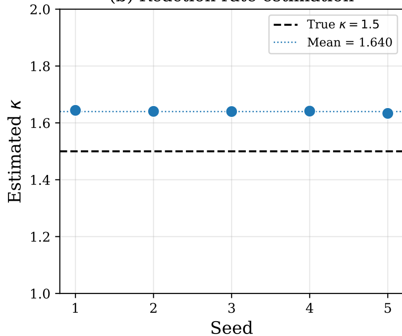
(b) Reaction rate estimation
