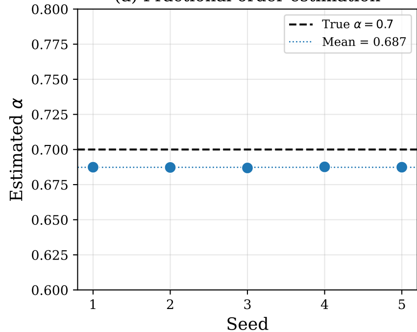
(a) Fractional order estimation
