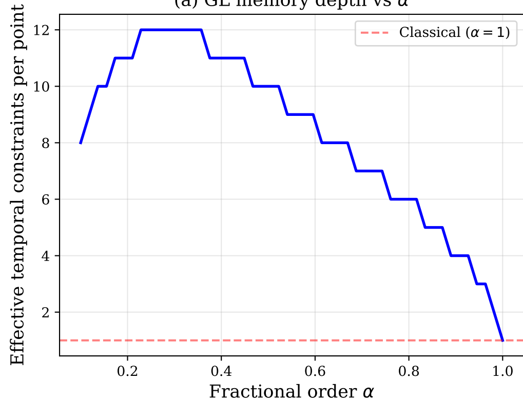
(a) GL memory depth vs \alpha
