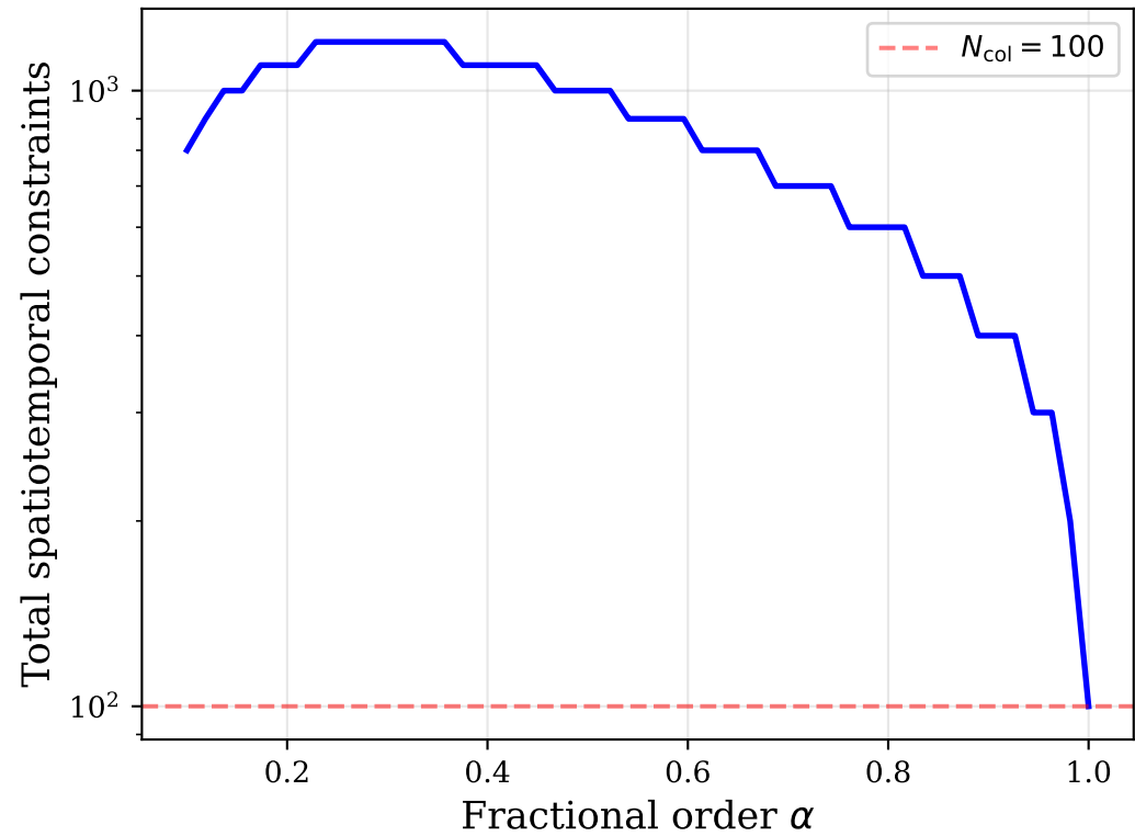
(b) Total constraints at N_{\text{col}} = 100
